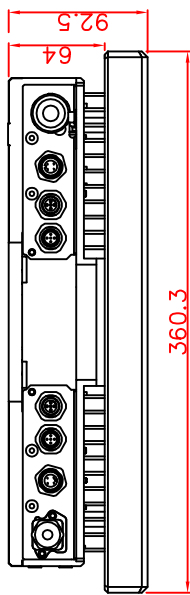
bottom view
