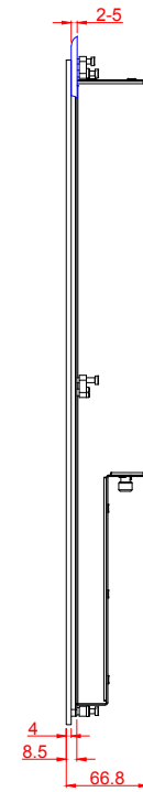
left view
