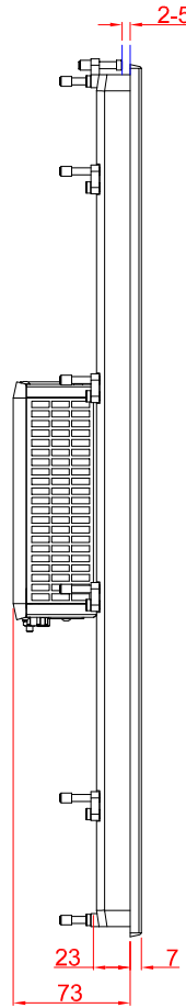
side view
