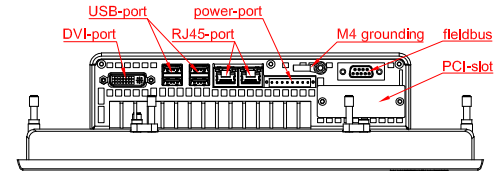
bottom view
