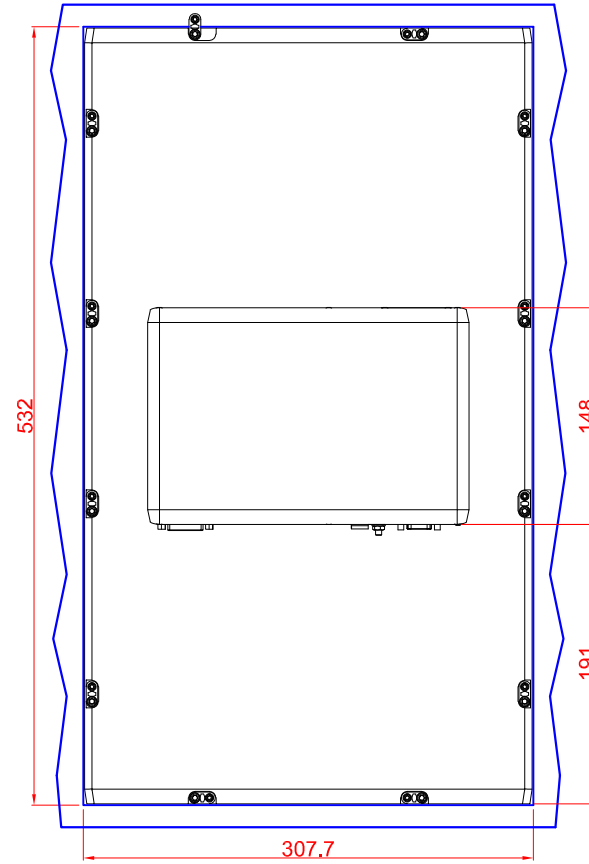
bottom view
