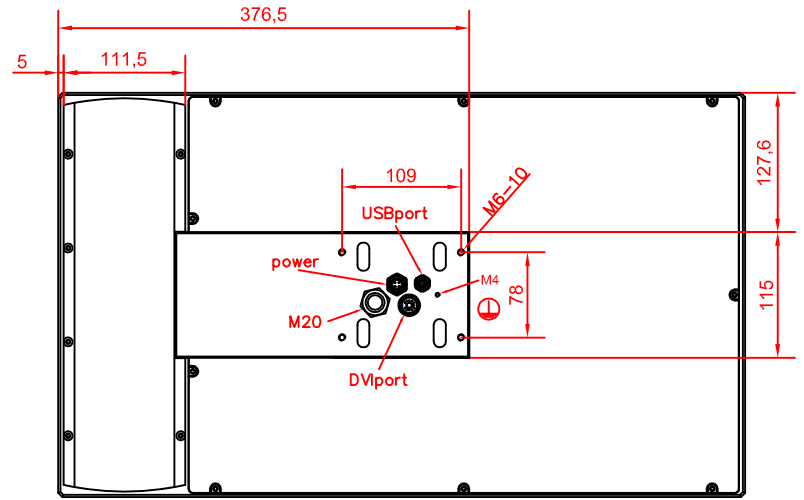
rear view
