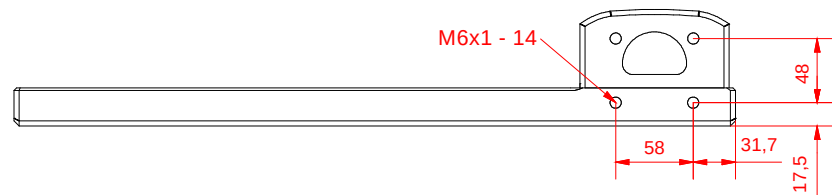
top view
