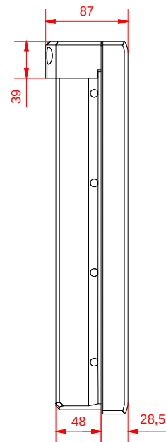
left view
