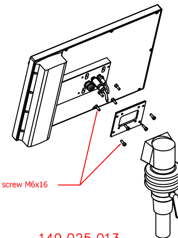
rear view
