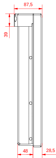
left view
