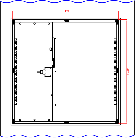
Rear view with inside measure
