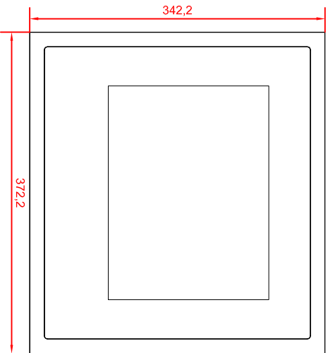
CP6911-0000 main dimensions
