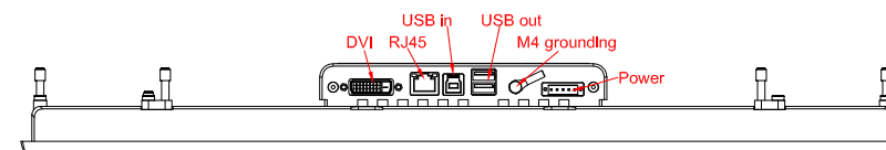
bottom view
