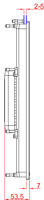
left view
