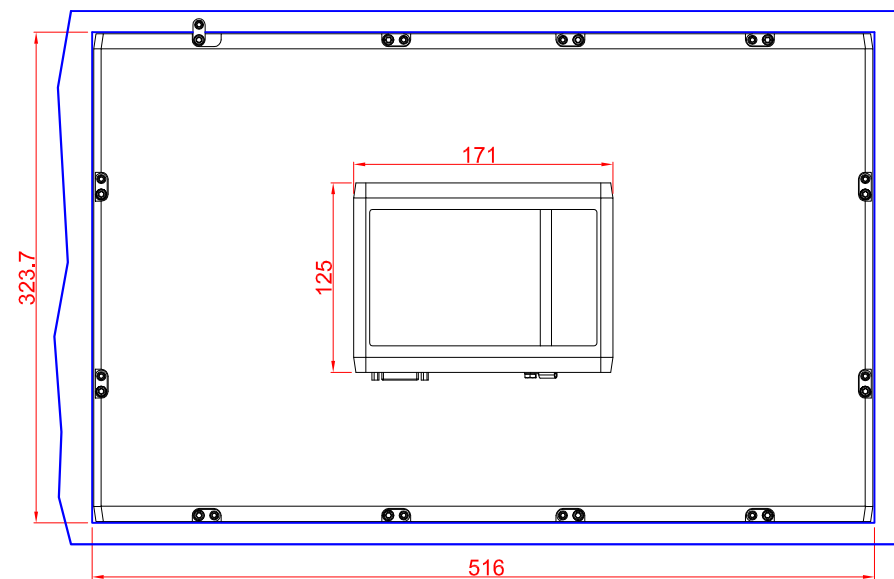
rear view
