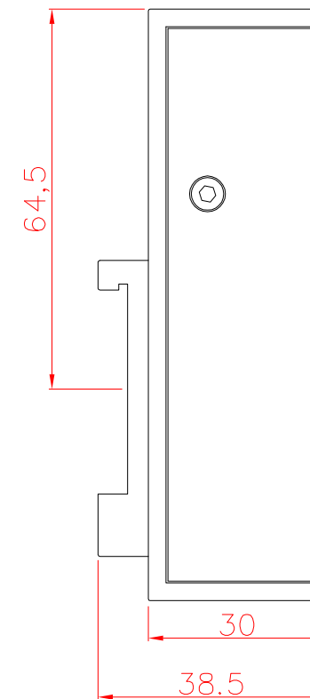
left view
