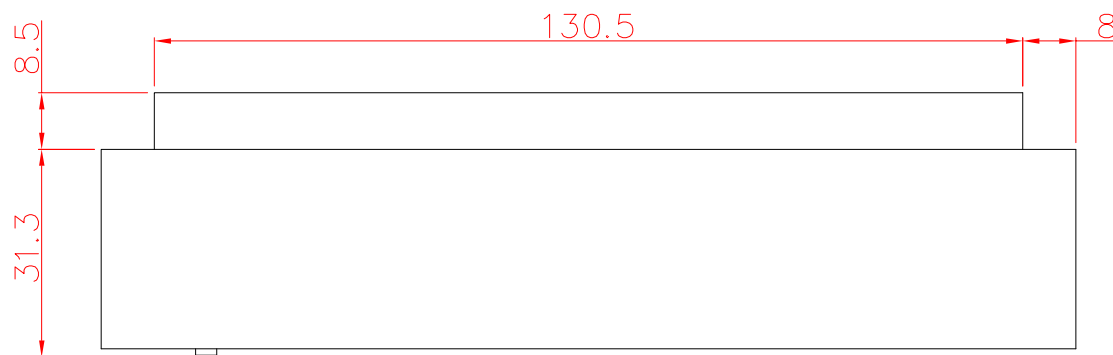
front view
