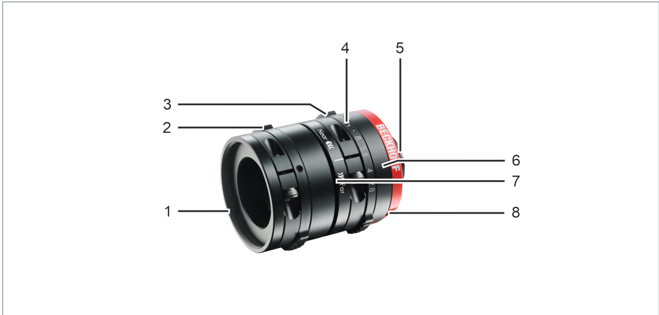
Fig. 2: VOS2000-5028 structure
