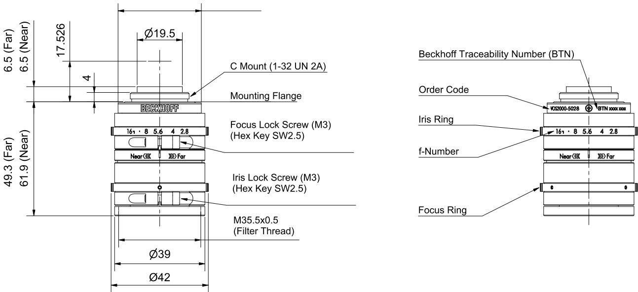
Fig. 3: Technical drawing
