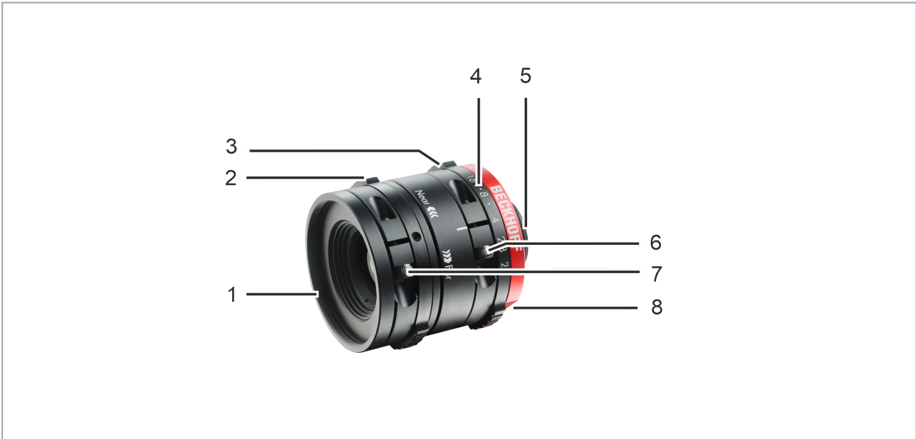
Fig. 2: VOS2000-0822 structure
