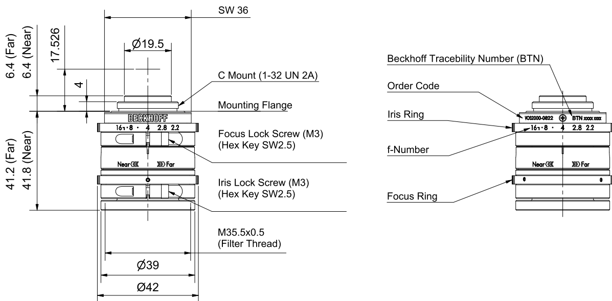
Fig. 3: Technical drawing
