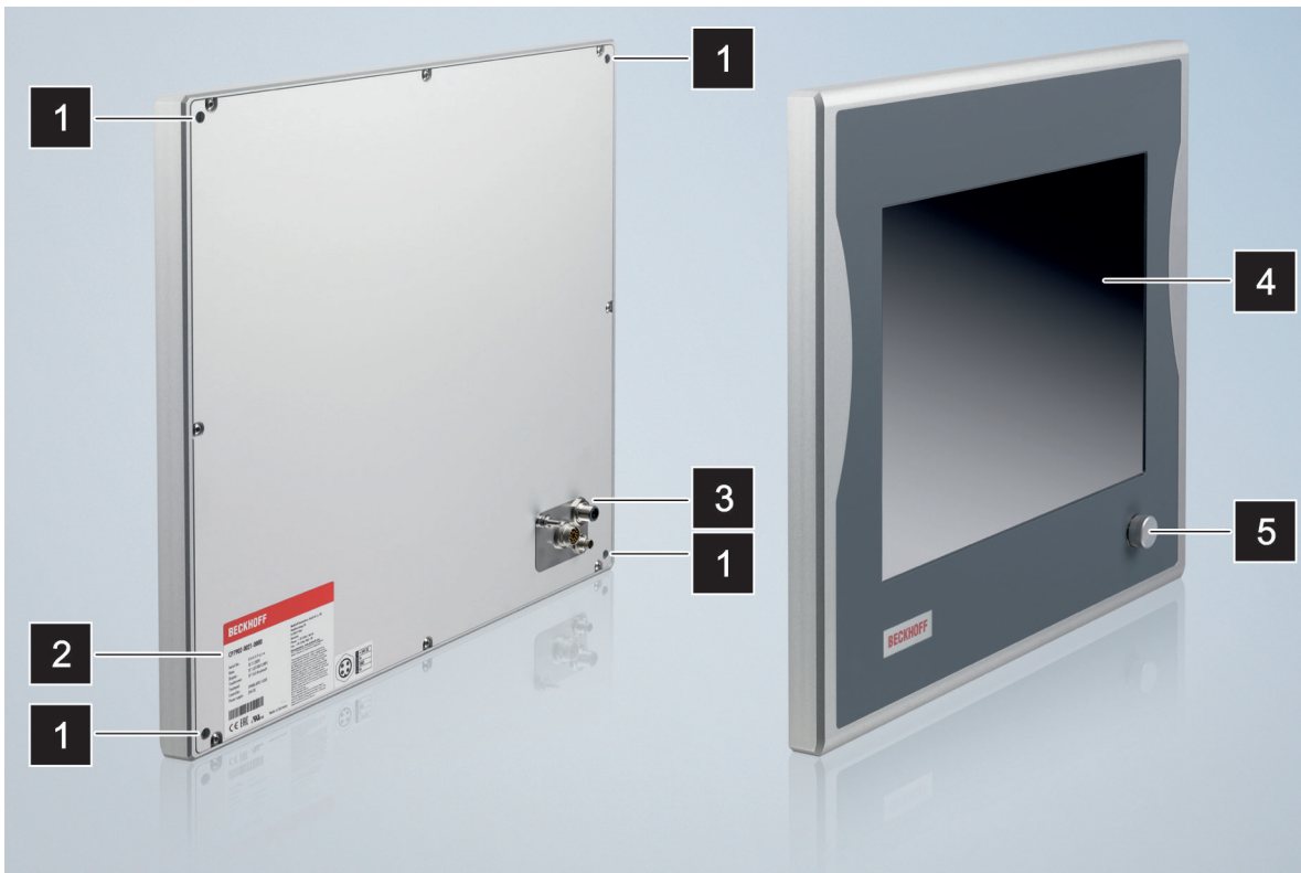
Fig. 1: Structure
