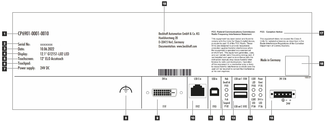
Fig. 9: Name plate
