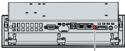
Abb. 7: CP6600_Status-LEDs
