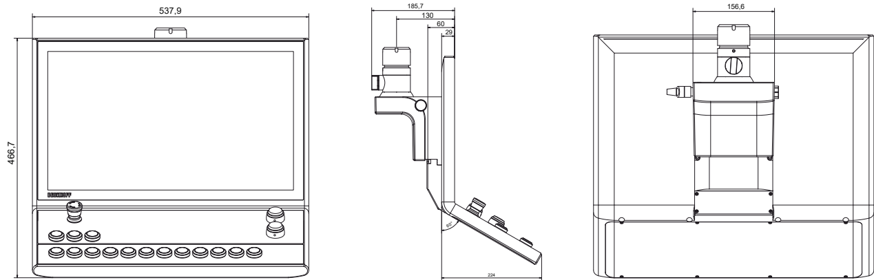
Fig. 23: Dimensions
