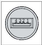
Fig. 10: USB interface pin numbering
