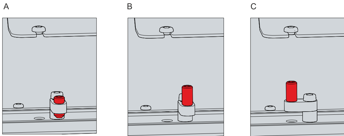
Fig. 19: Removal from the control cabinet
