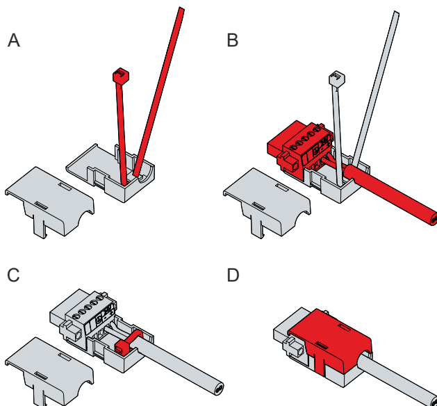
Fig. 16: Assembly of strain relief housing
