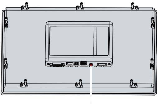
Fig. 18: Grounding bolt for functional earthing
