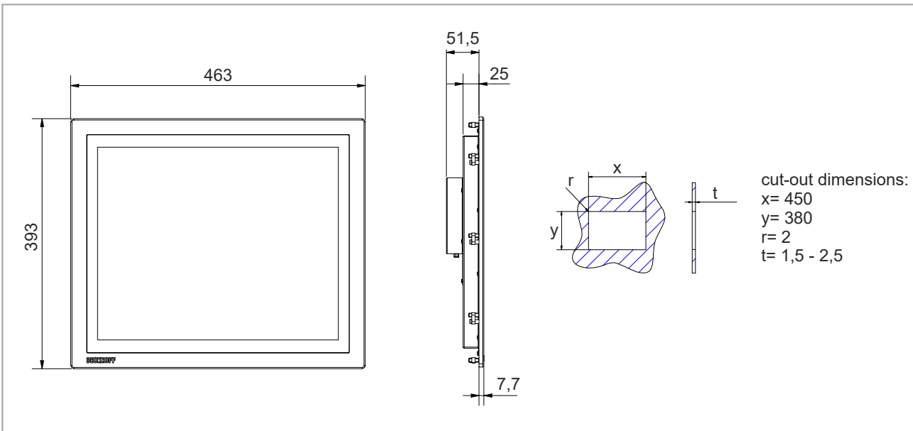
Fig. 8: Dimensions 19-inch
