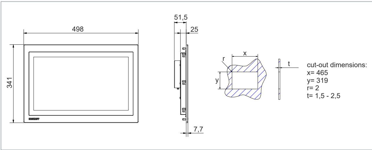
Fig. 7: Dimensions 18.5-inch
