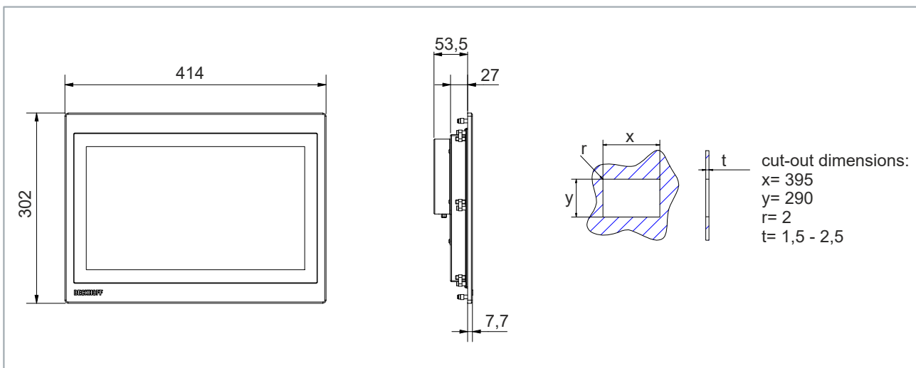
Fig. 6: Dimensions 15.6-inch
