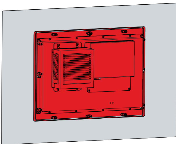
Fig. 20: Removal installation cutout
