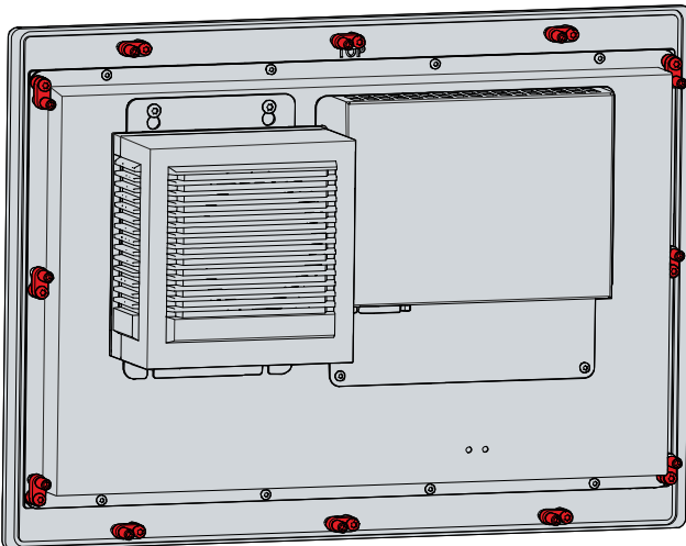
Fig. 13: Delivery state clamping lever
