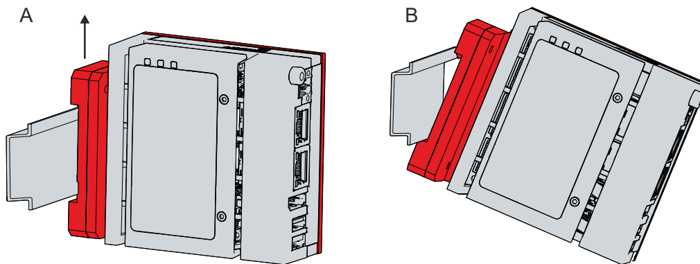
Abb. 23: Demontage Hutschienenadapter
