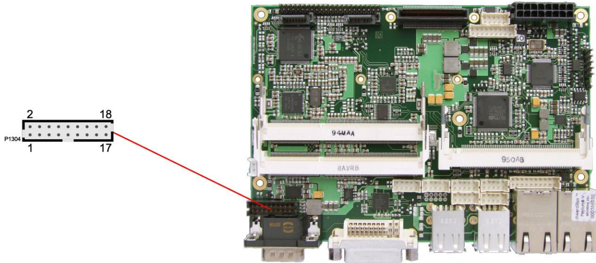
Pinout 2x9pin connector DVI/HDMI:
