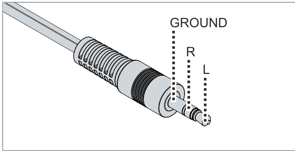
Abb. 10: Klinkenstecker Line In / Line Out X300, X302.
