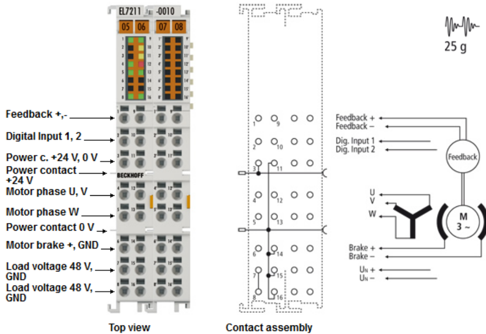
Abb. 5: EL7211-0010
