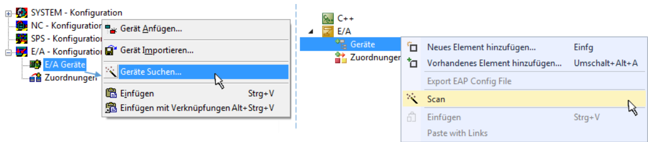
Abb. 65: Scan Devices (links: TwinCAT 2; rechts: TwinCAT 3)
