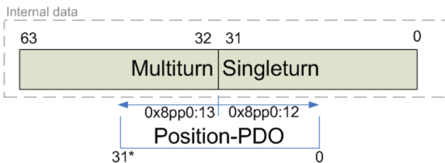
Abb. 114: Multiturn / Singleturn bits
