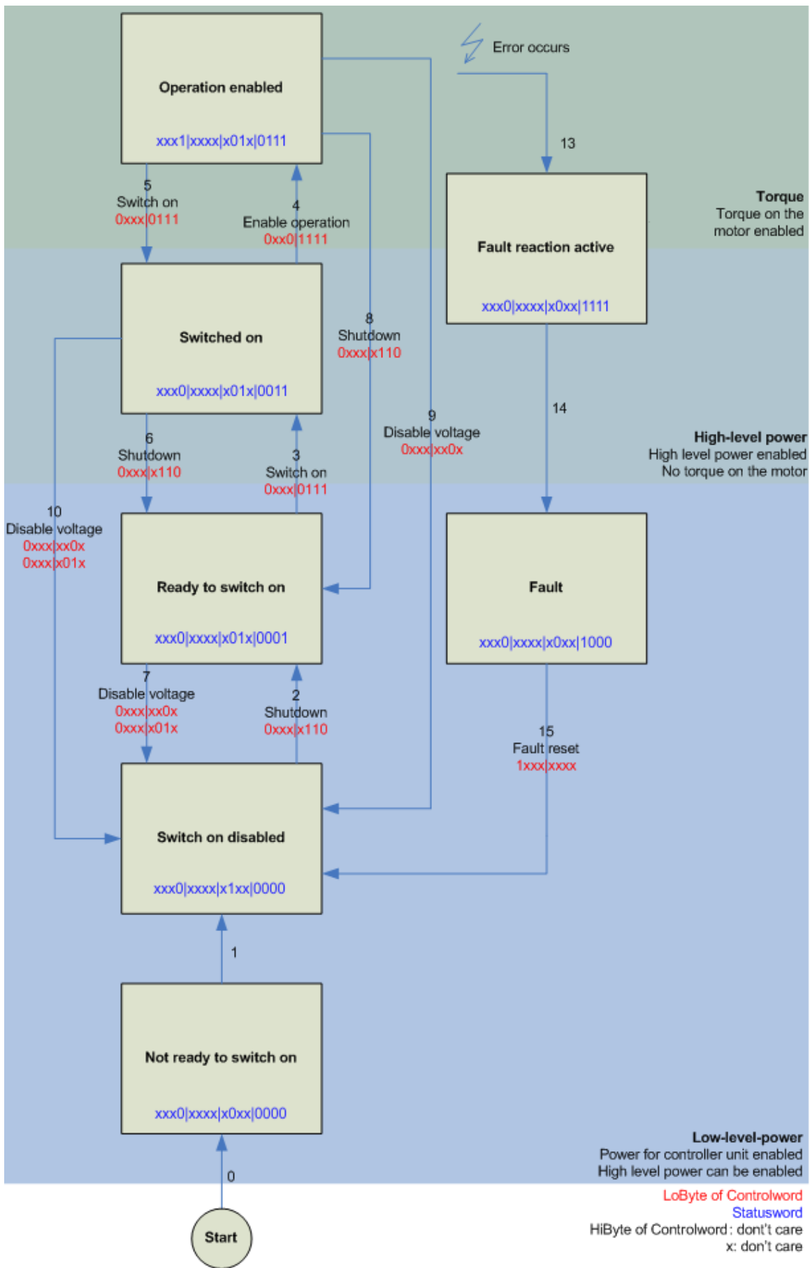
Abb. 123: DS402 State Machine
