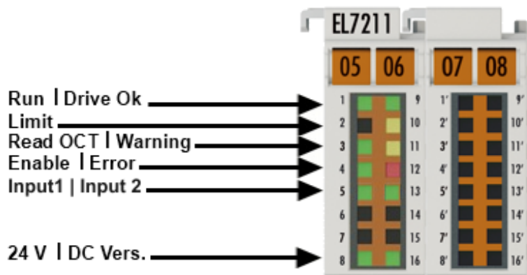
Abb. 35: EL7211-001x - LEDs
