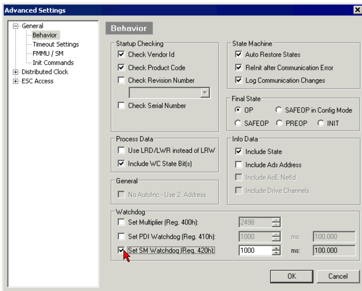
附图 6: EtherCAT 选项卡 -&gt; Advanced Settings -&gt; Behavior-&gt; Watchdog
