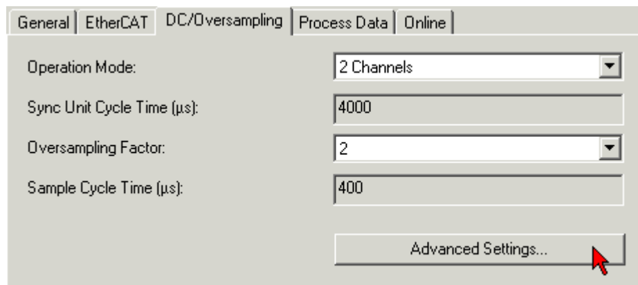
附图 185: DC 选项卡，激活“Advanced Settings...（高级设置...）”，TwinCAT 2.11
