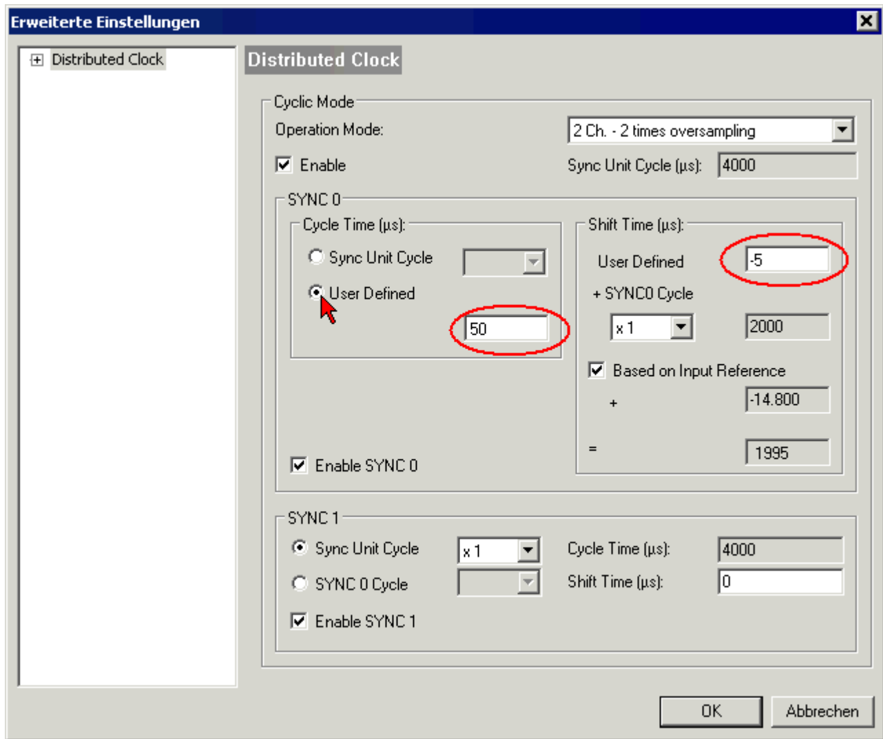
附图 186: DC 选项卡，激活“Advanced Settings... (高级设置...)”，“Distributed Clocks (分布式时钟)”
