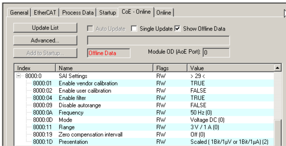
Abb. 149: Reiter CoE - Online, TwinCAT System Manager
