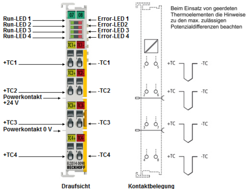
Abb. 62: EL3314-0090
