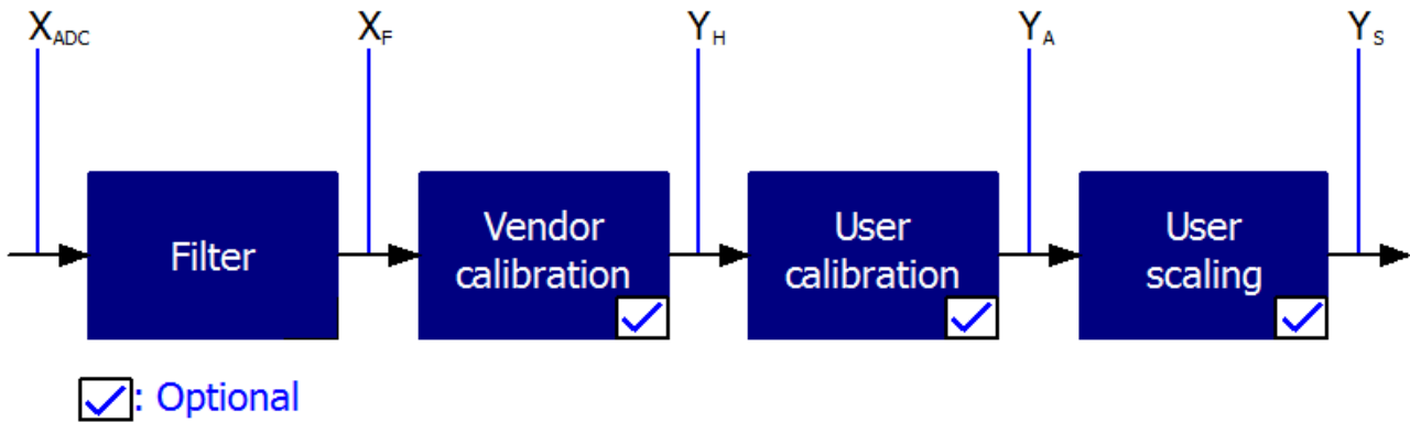
Fig. 226: Calculation of process data
