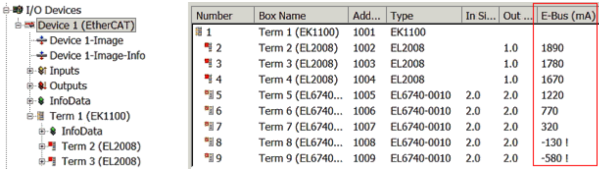
Fig. 82: System manager current calculation
