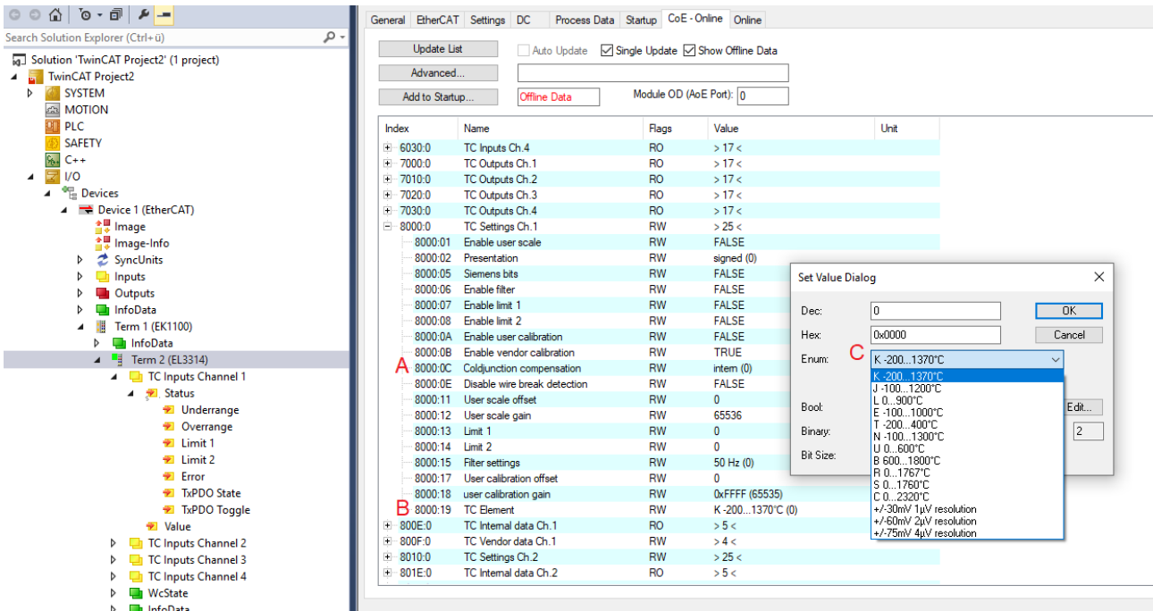
Fig. 211: Setting the measuring range
