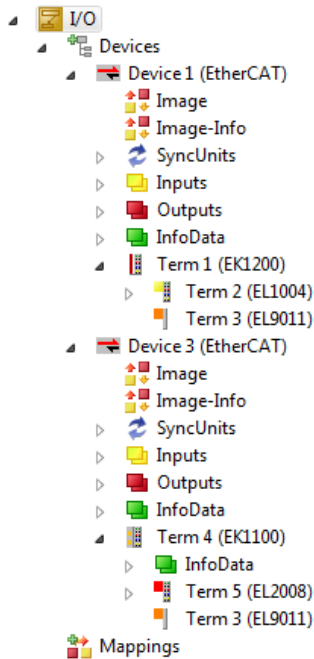
Fig. 128: Mapping of the configuration in VS shell of the TwinCAT 3 environment
