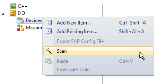
Fig. 126: Select “Scan”
