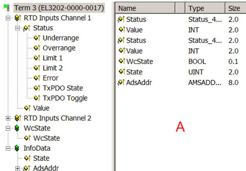
Fig. 216: EL32xx-0000-0017 process image in the TwinCAT 2.11 representation
