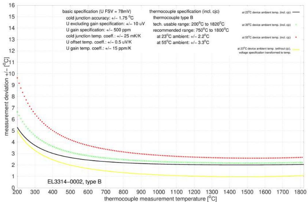
Fig. 11: EL3314-0002 and EL3314-0092 (corresponds to EL3314-0002), type B
