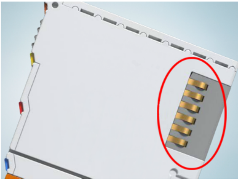
Fig. 89: Spring contacts of the Beckhoff I/O components
