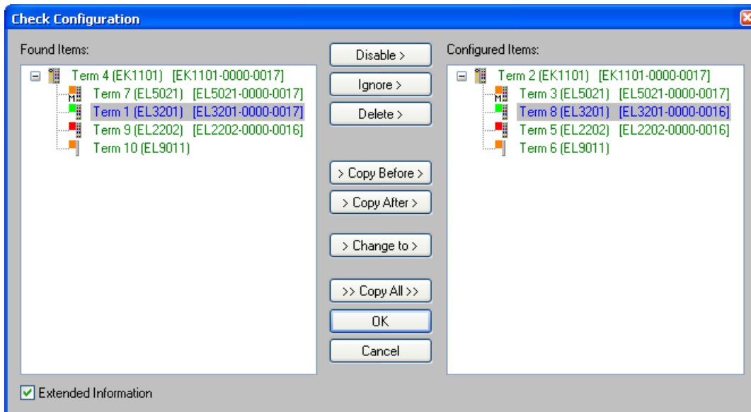
Fig. 220: Typical result after scanning an EtherCAT system
