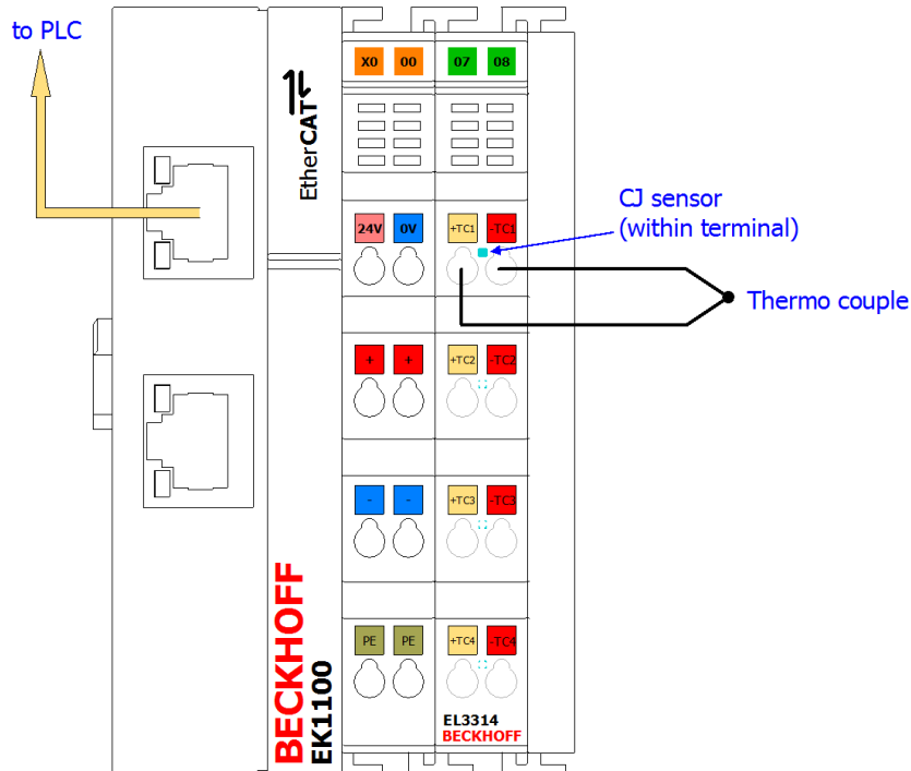
Fig. 241: Structure of the sample program for "separate temperature calculation with CJC in the PLC"
