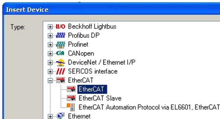
Fig. 162: Selecting the EtherCAT connection (TwinCAT 2.11, TwinCAT 3)
