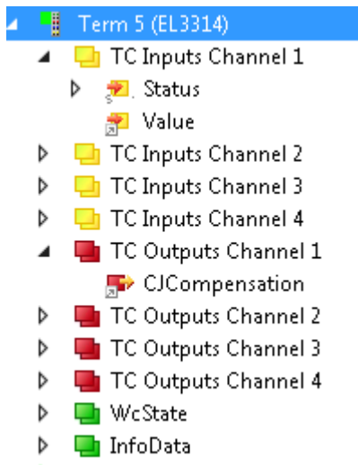
Fig. 230: Display of the "Value" in the TwinCAT tree
