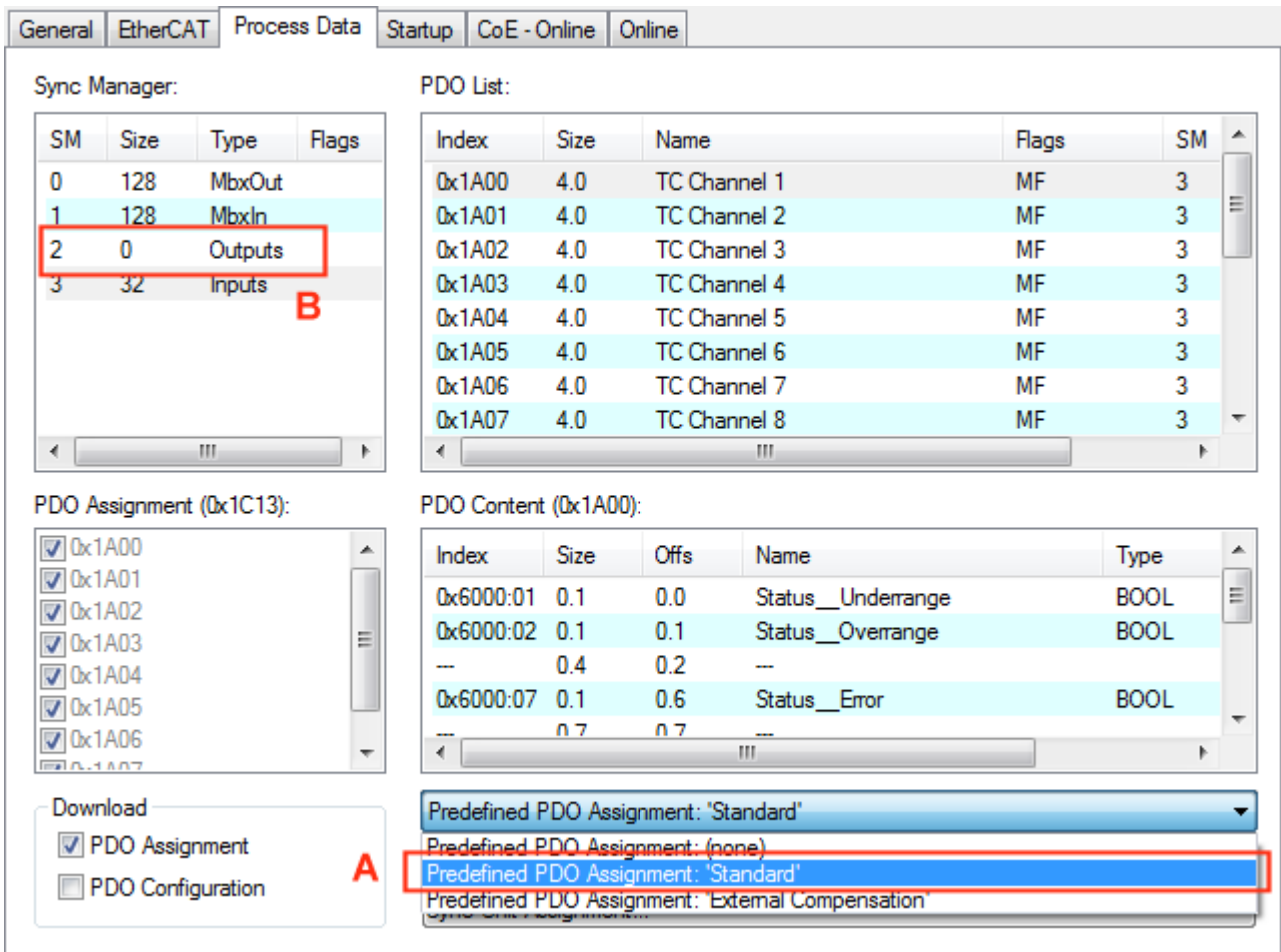
Fig. 212: TwinCAT System Manager with predefined PDO option "Standard"
