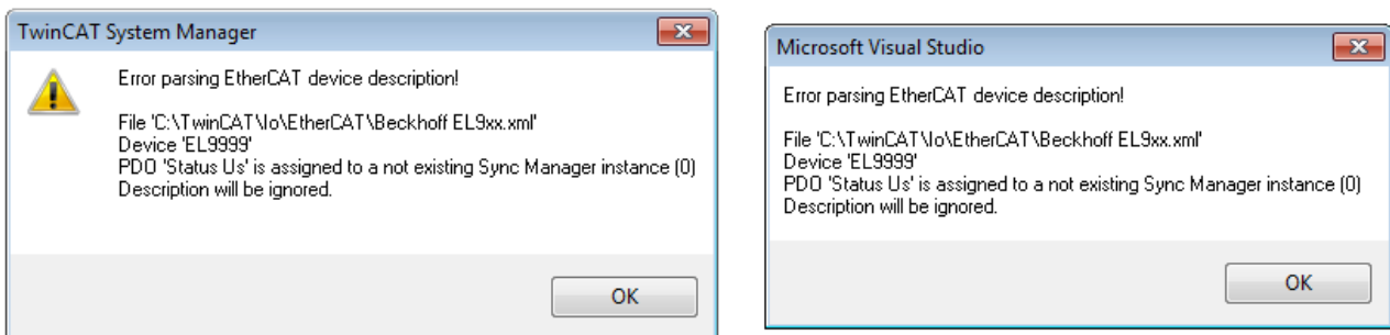
Fig. 158: Information window for faulty ESI file (left: TwinCAT 2; right: TwinCAT 3)
