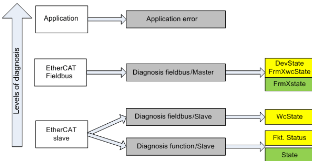
Fig. 202: Selection of the diagnostic information of an EtherCAT Slave
