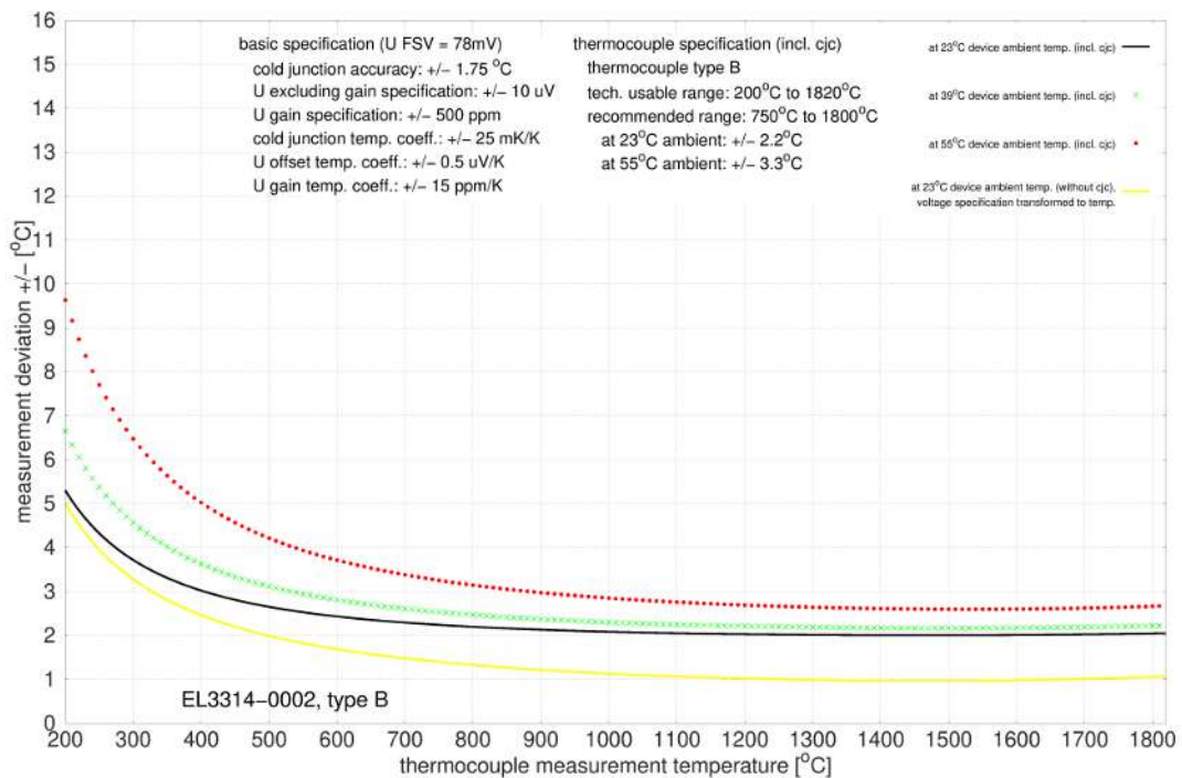
Fig. 65: EL3314-0002 and EL3314-0092 (corresponds to EL3314-0002), type B
