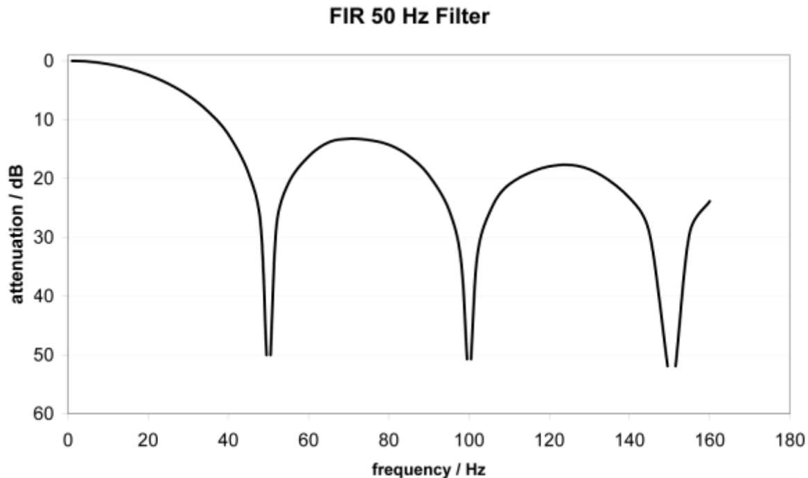
Fig. 225: Example notch filter
