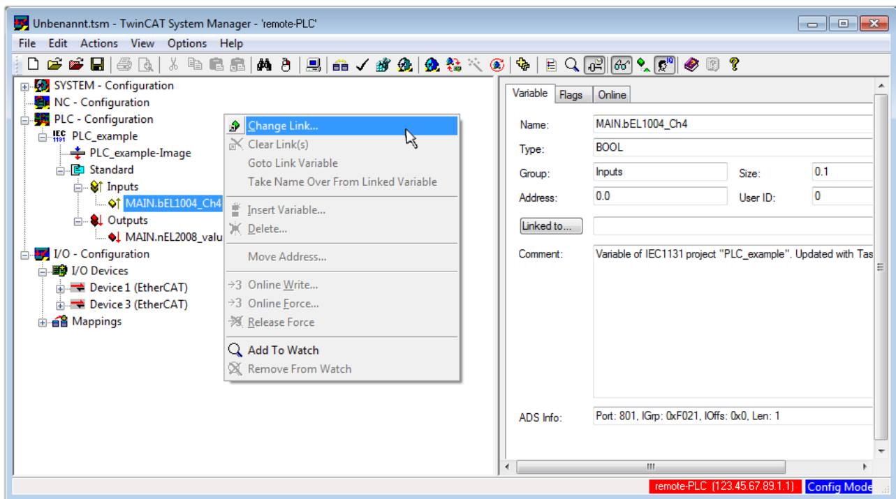
Fig. 115: Creating the links between PLC variables and process objects
