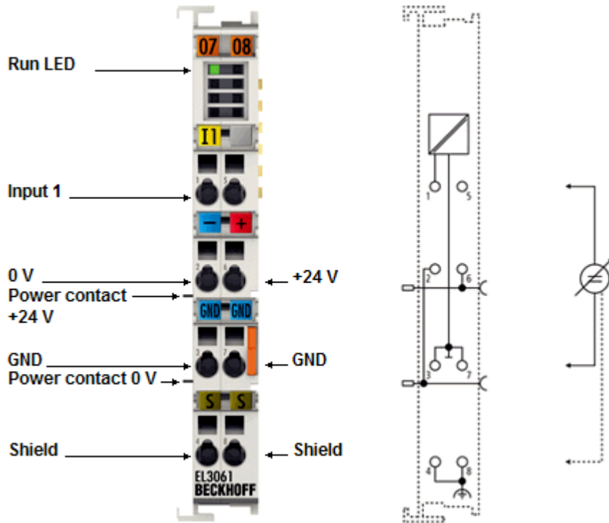
附图 41: EL3061 RUN LED
