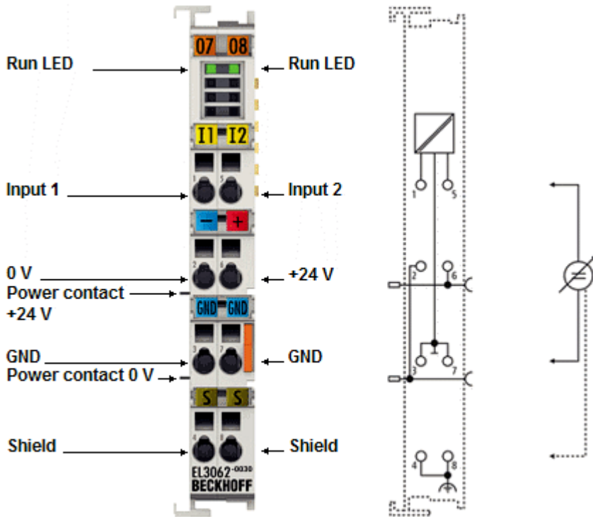
附图 45: EL3062-0030 RUN LED
