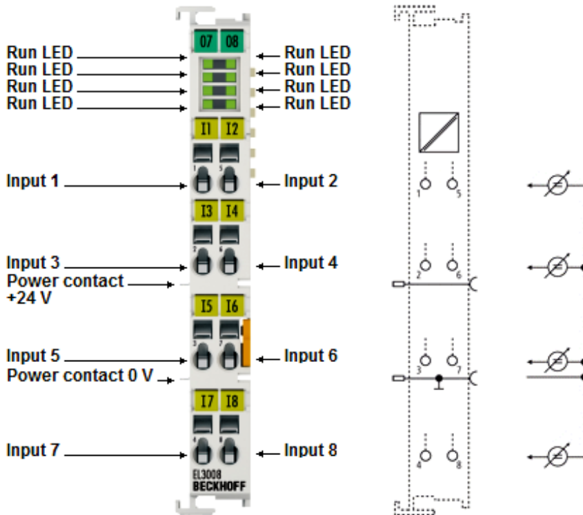
附图 11: LED EL3008
