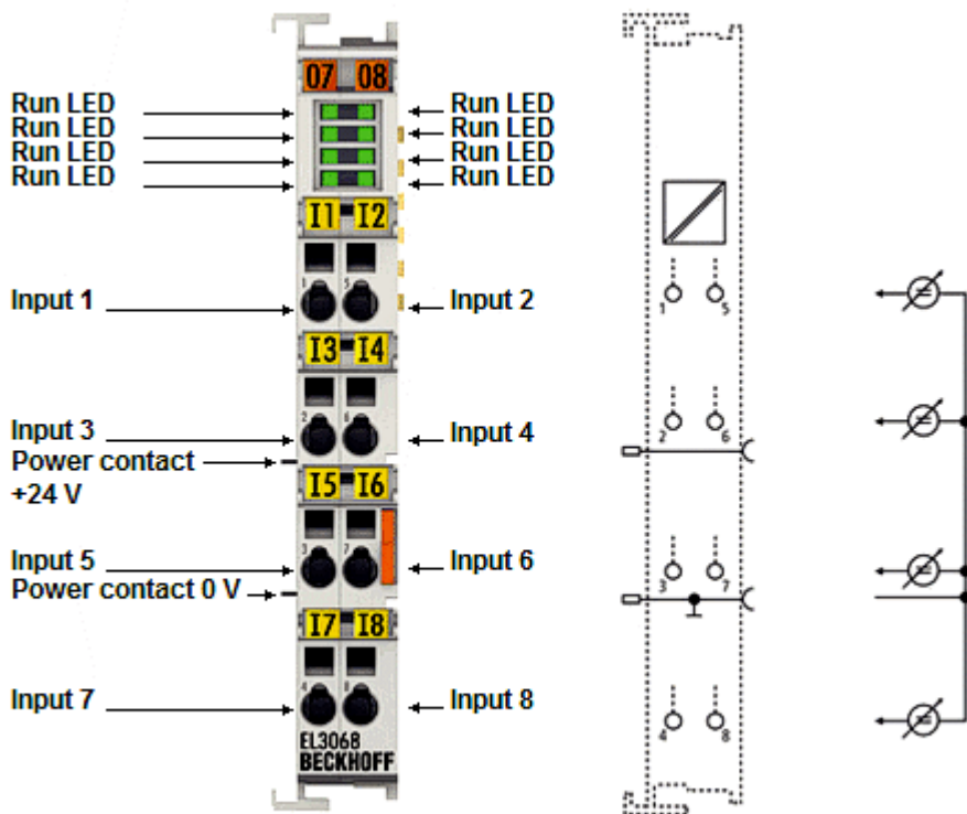
附图 49: EL3068 RUN LED
