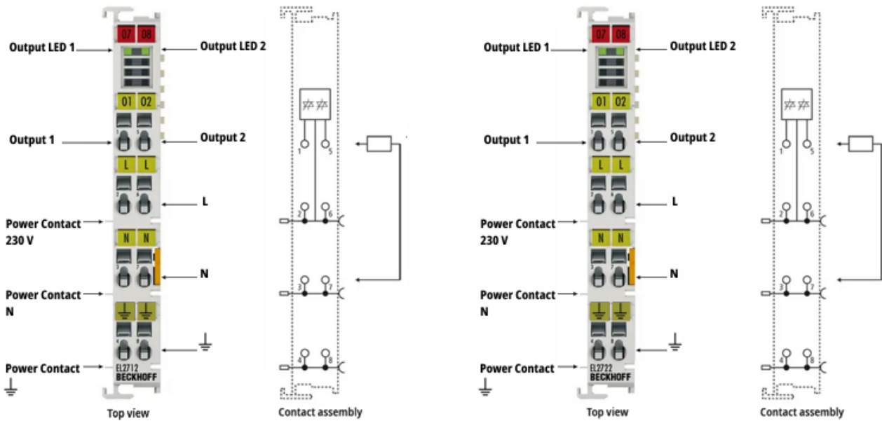
Abb. 5: EL2712, EL2722
