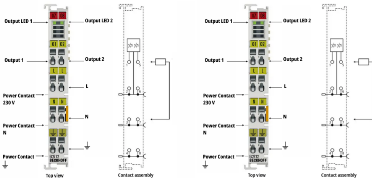
Abb. 4: EL2712, EL2722
