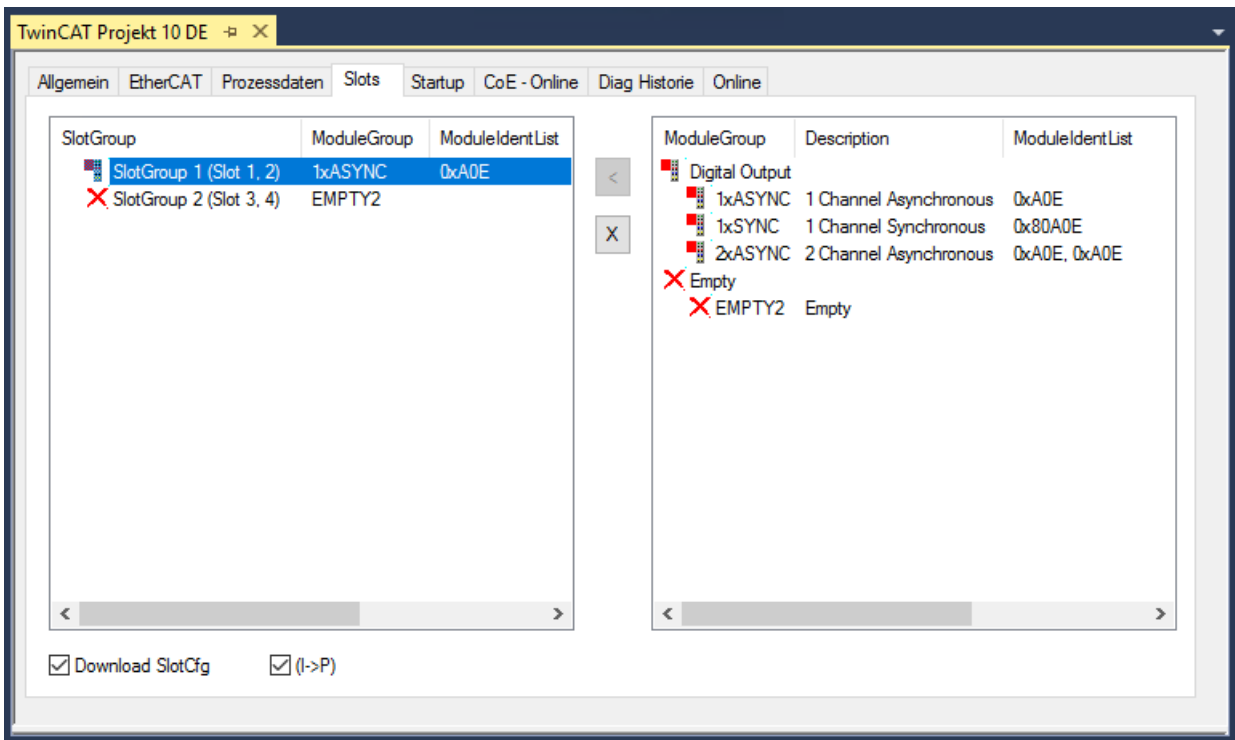
Abb. 127: EL2574 - Reiter Slots
