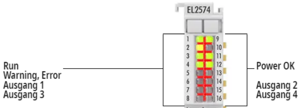
Abb. 5: EL2574 LEDs
