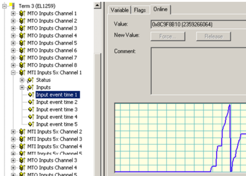
Fig. 168: Timestamp via online display
