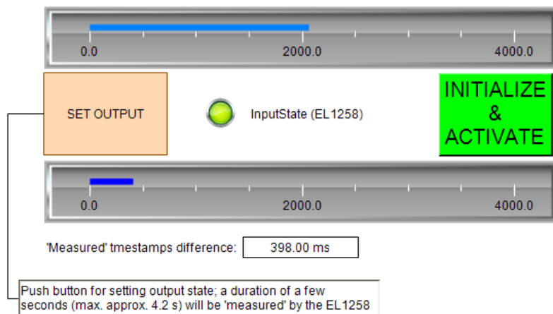
Fig. 184: Sample program EL1258 / Visualization_1: simple time measurement based on two state changes
