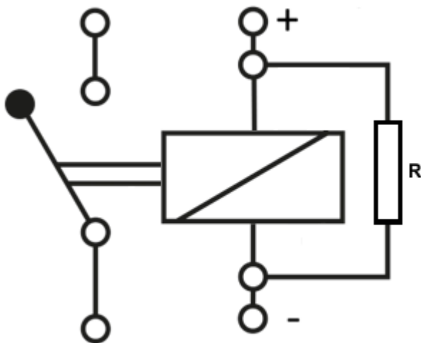
Fig. 31: Resistance parallel to inductance
