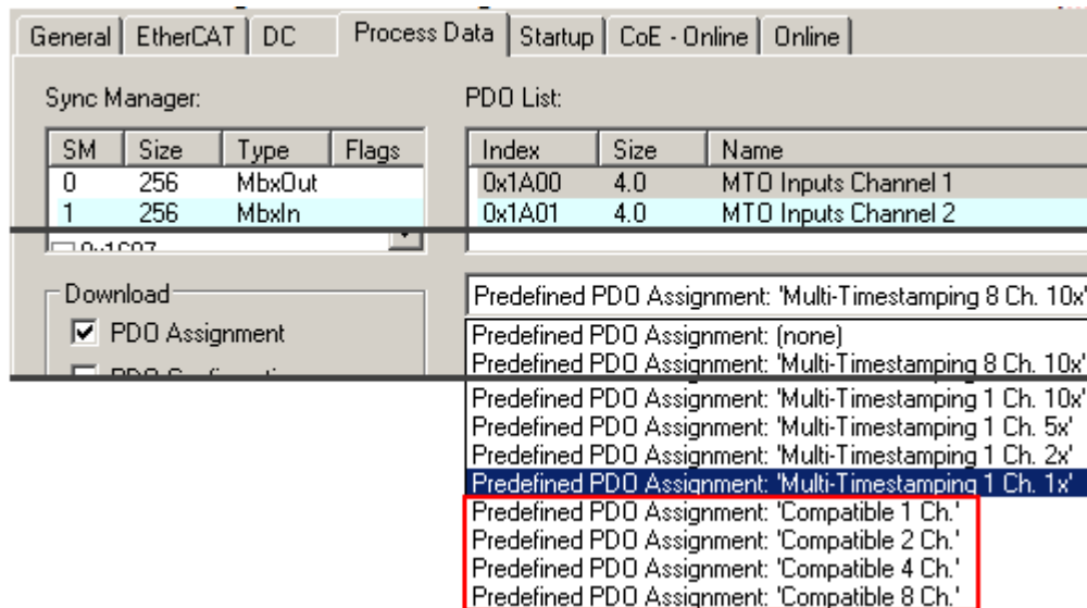
Fig. 175: Predefined PDOs for compatibility mode
