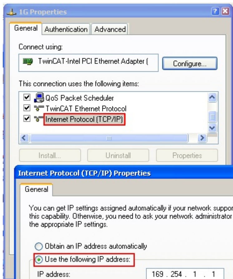
Fig. 96: TCP/IP setting for the Ethernet port
