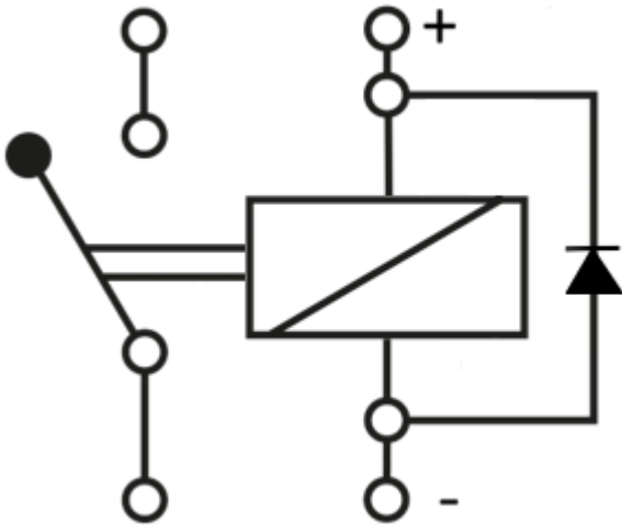
Fig. 32: Short-circuit diode on the inductance, free-wheeling diode
