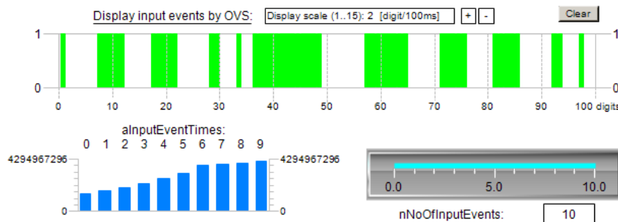
Fig. 185: Sample program EL1258 / Visualization_2: Display of incoming events in chronological order according to the timestamps of the EL1258
