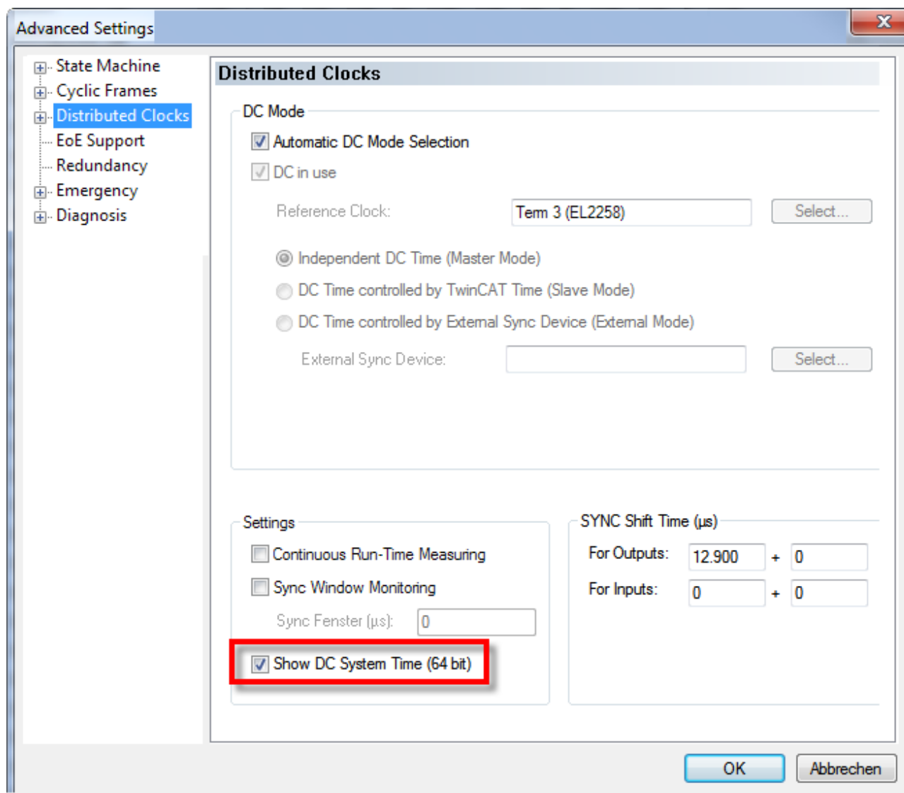
Fig. 176: Activation of the master distributed clock display
