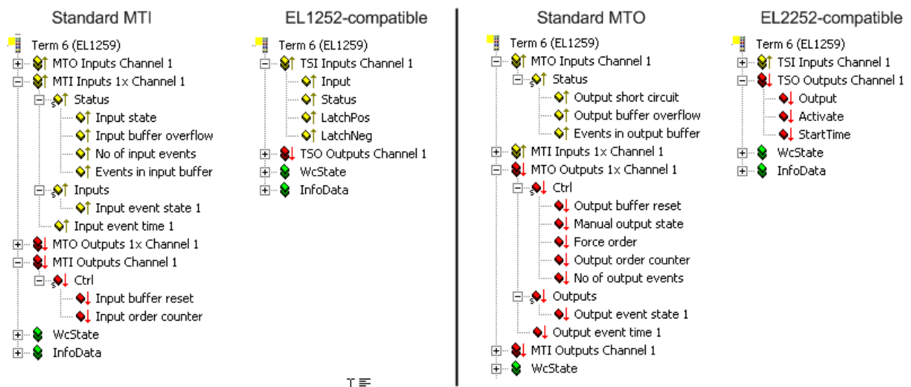
Fig. 157: Option for setting of compatibility modes in relation to EL1252/EL2252
