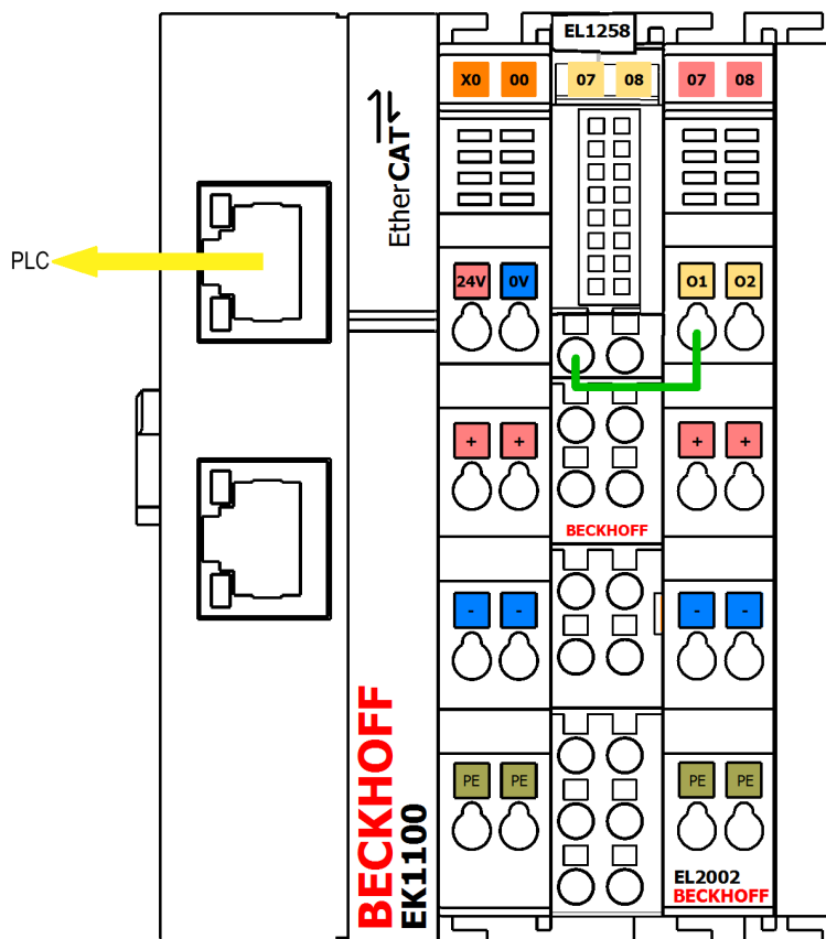
Fig. 182: Recommended structure for the EL1258 sample program
