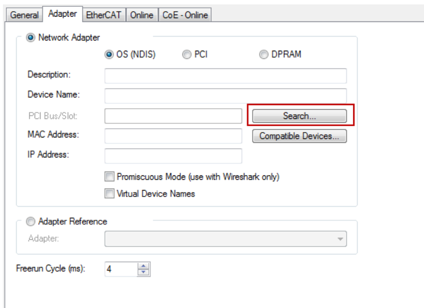
Fig. 180: Search of the existing HW configuration for the EtherCAT configuration of the example
