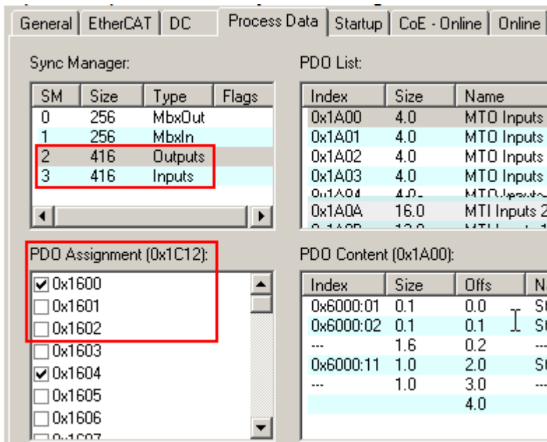
Fig. 159: Free selection of the PDO
