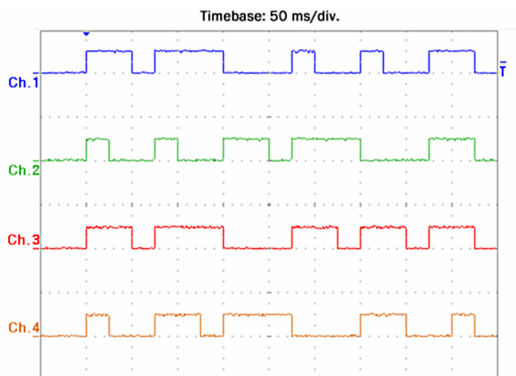
Fig. 181: Recording of four channels by the Multi-Timestamp program example
