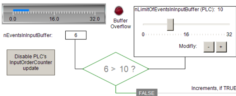
Fig. 186: Query of the "EventInInputBuffer" of the EL1258: Are there any other events stored in the terminal?
