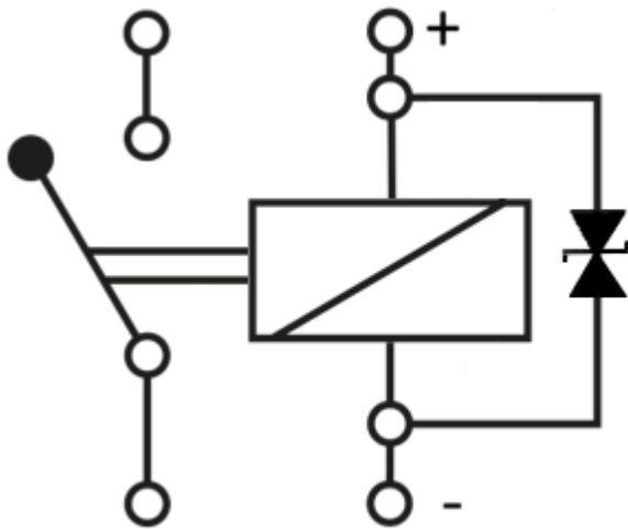
Fig. 34: Example circuit with bidirectional suppressor diode (Transient Voltage Suppressor)
