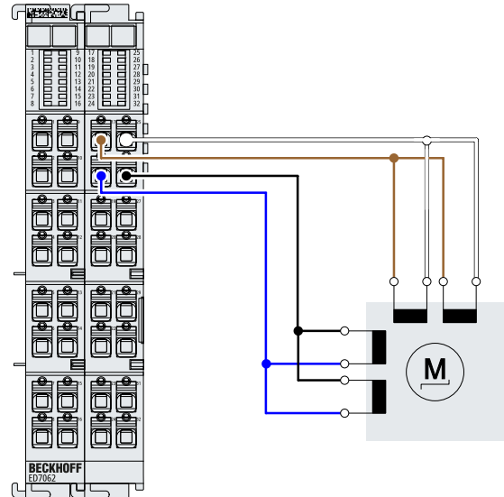
Parallel connection
