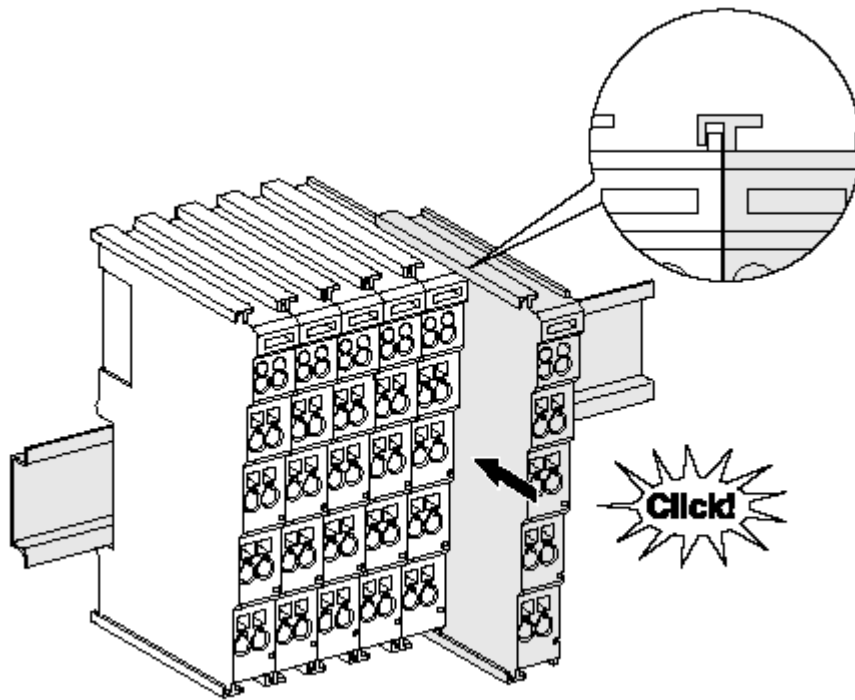
Fig. 2: Installation on the mounting rail
