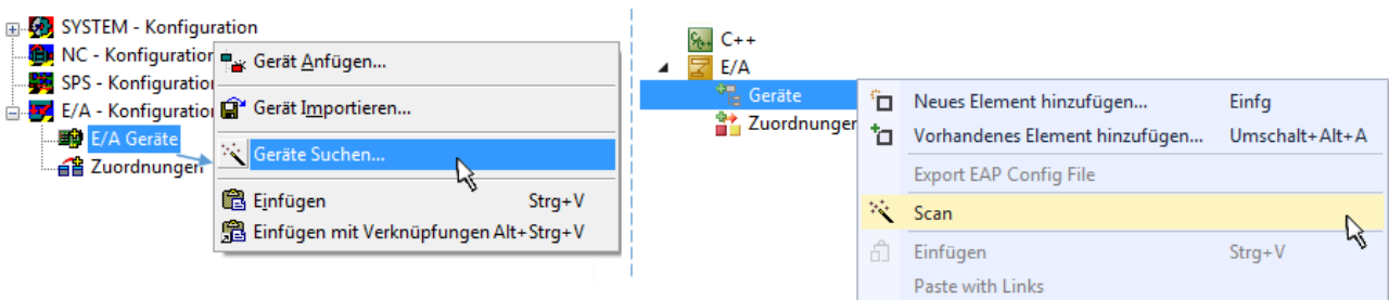
Abb. 122: Scan Devices (links: TwinCAT 2; rechts: TwinCAT 3)
