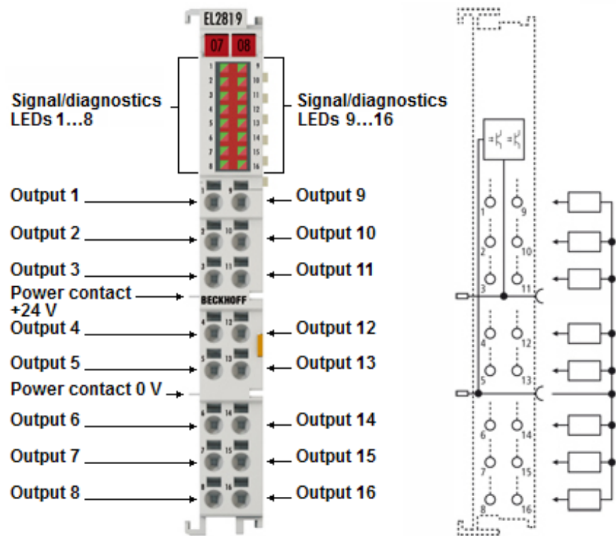
Abb. 14: EL2819
