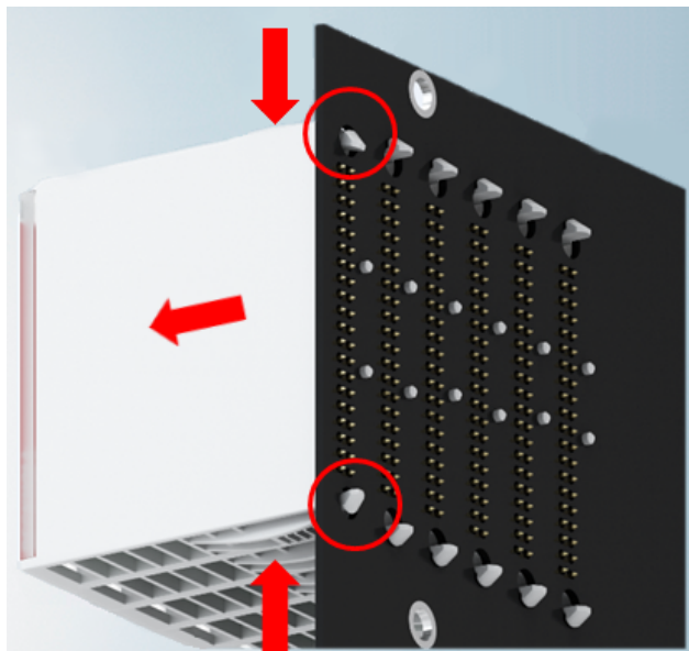
Fig. 30: Disassembly of EJ modules
