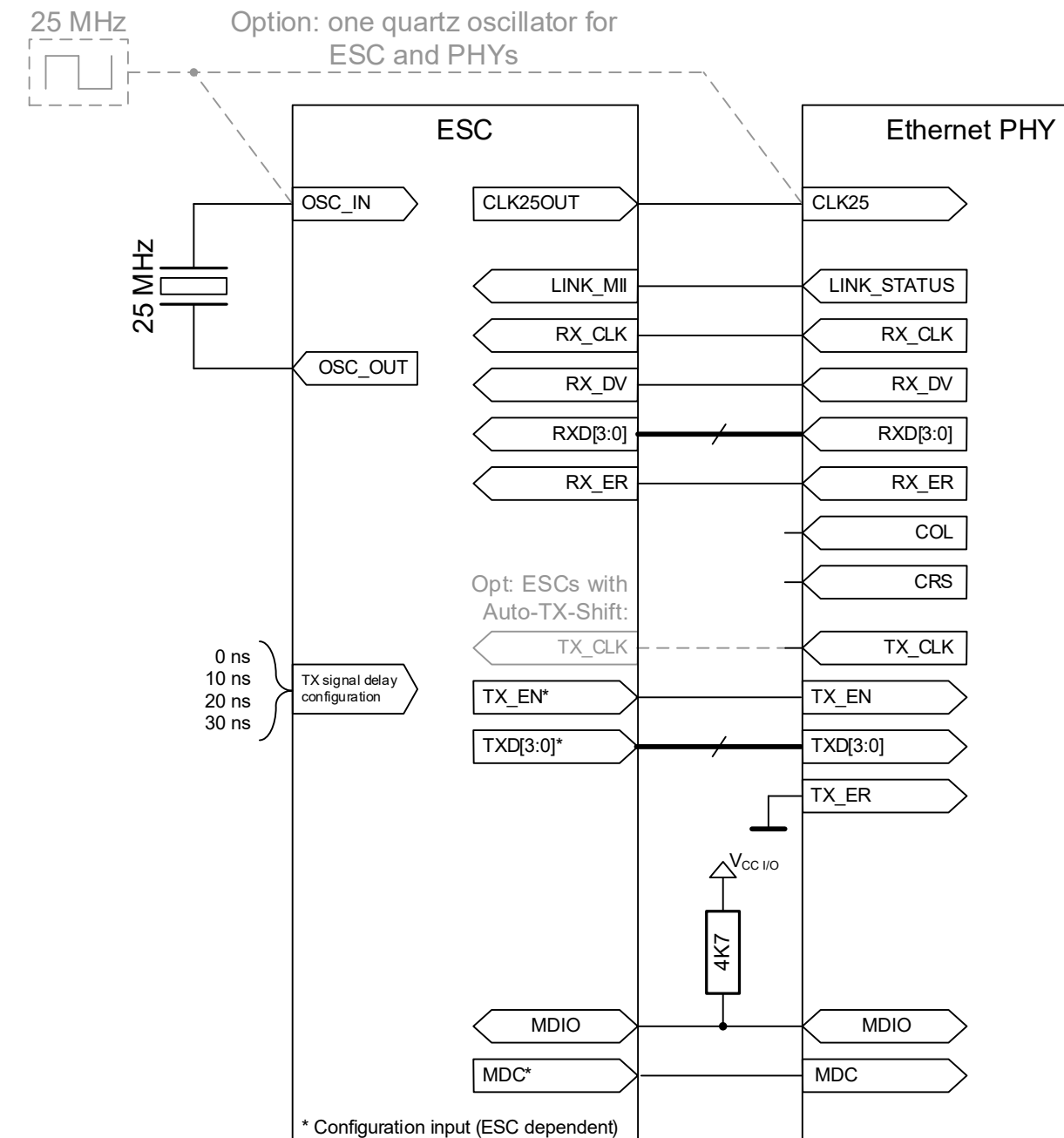
Figure 2: PHY connection (MII)
