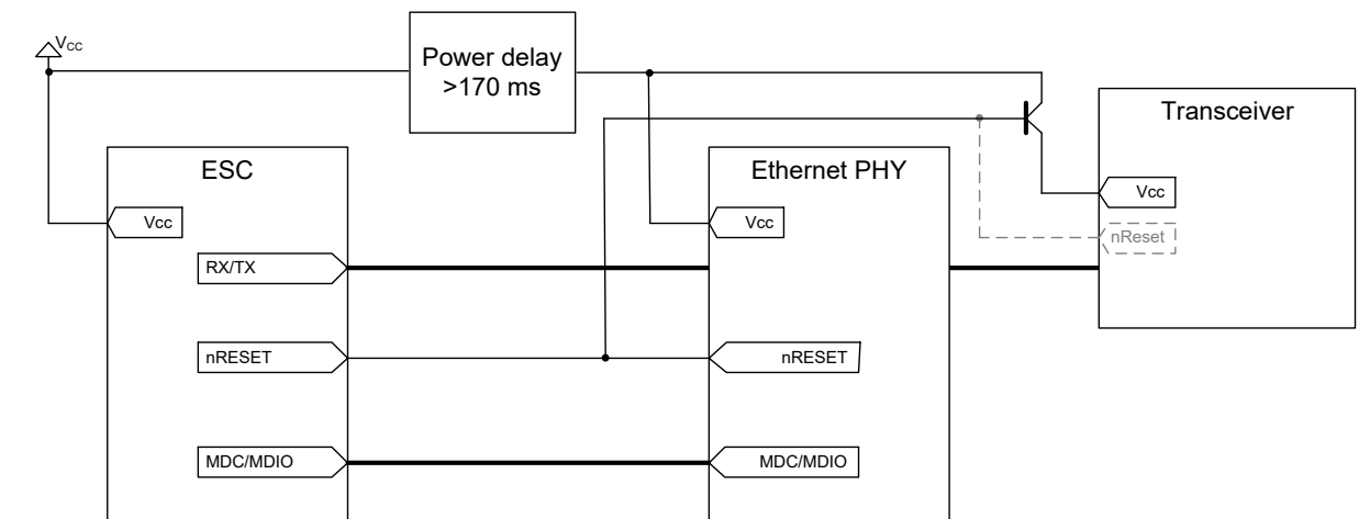
Figure 5: PHY power sequencing with transceiver power down/reset
