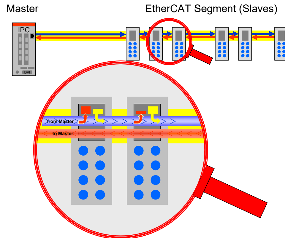
Figure 1: EtherCAT segment
