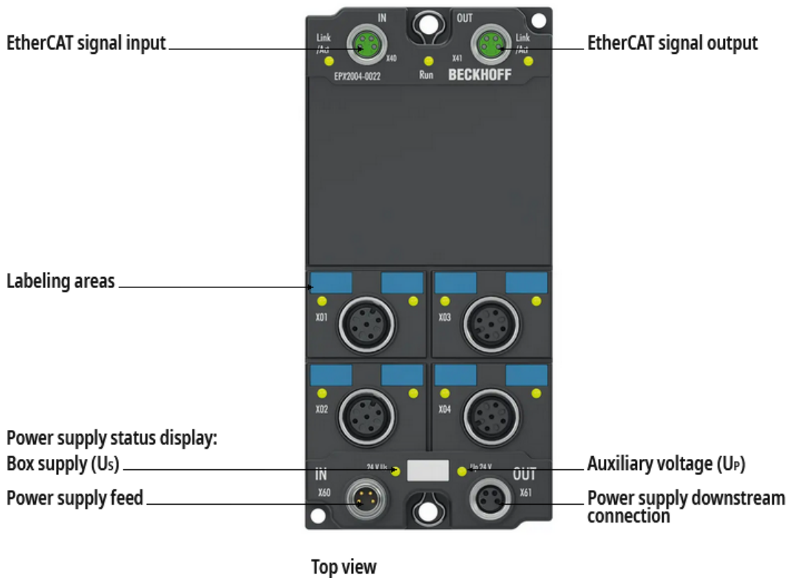
Fig. 2: EPX2004-0022 - EtherCAT Box, 4-channel digital input/output, 24 V DC, 50 mA, M12, Ex i
