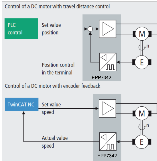
Fig. 1: Implementation options for control loops with EPP7342-0002
