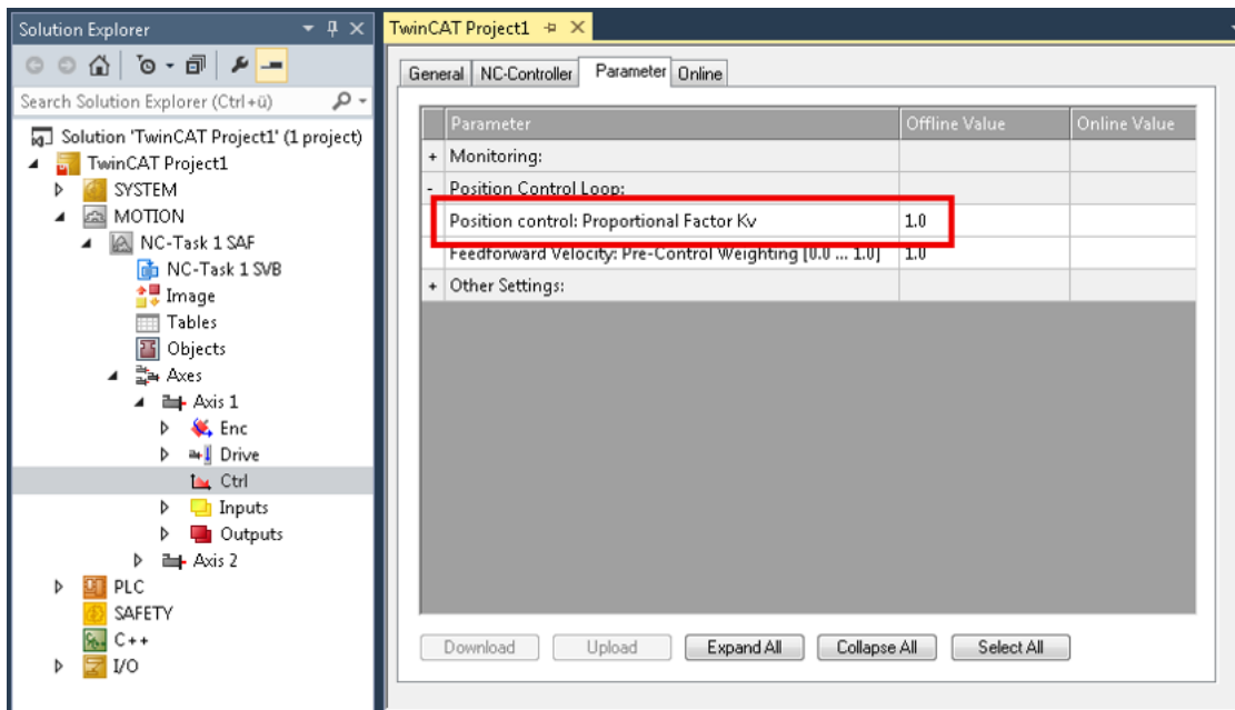
Fig. 19: Setting the proportional factor K_v
