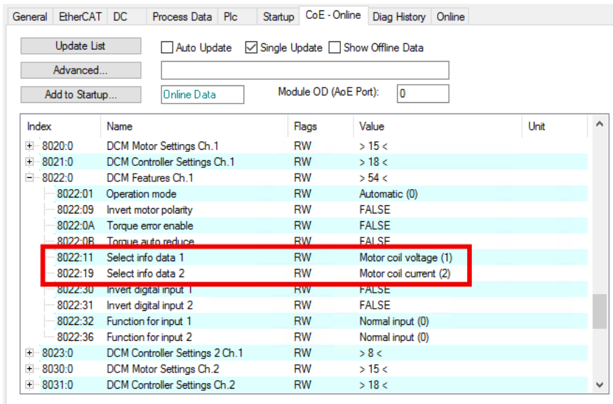
Fig. 10: Selection of additional information data
