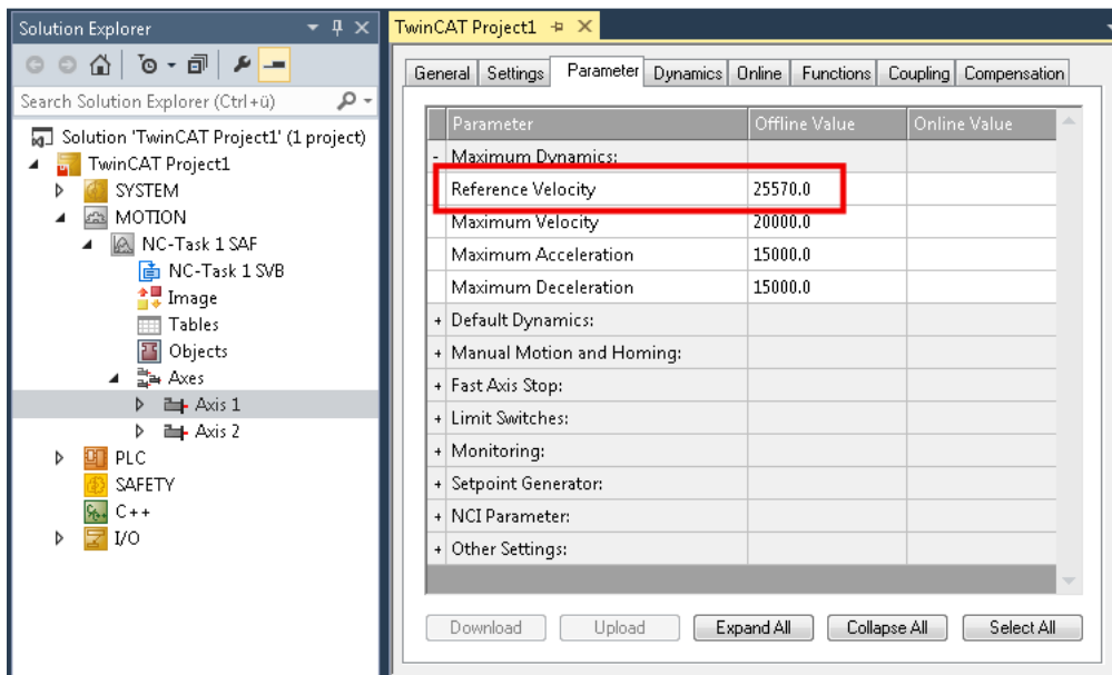
Fig. 14: Reference velocity selection
