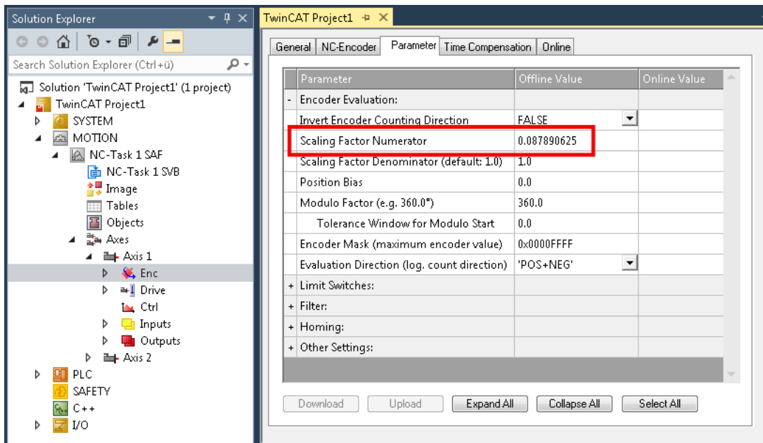
Fig. 16: Setting the Scaling Factor
