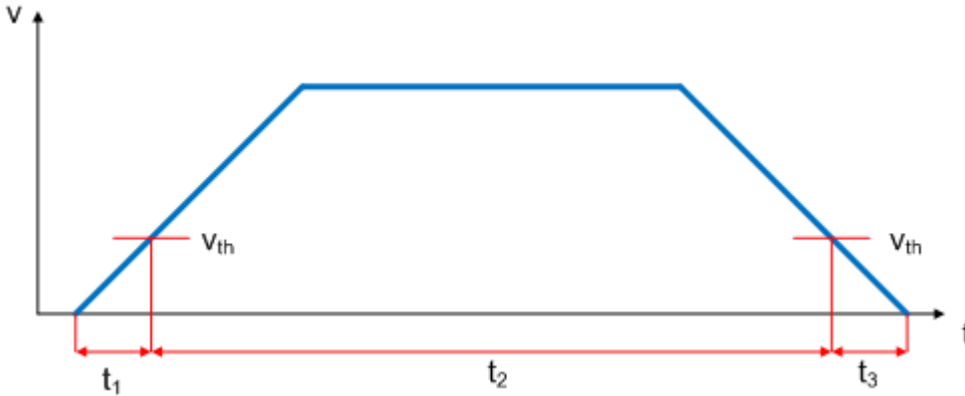
Fig. 18: Velocity ramp with K_v factor limit values
