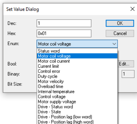
Fig. 11: Dialog box
