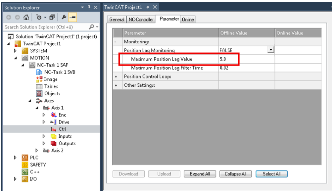
Fig. 17: Position lag monitoring
