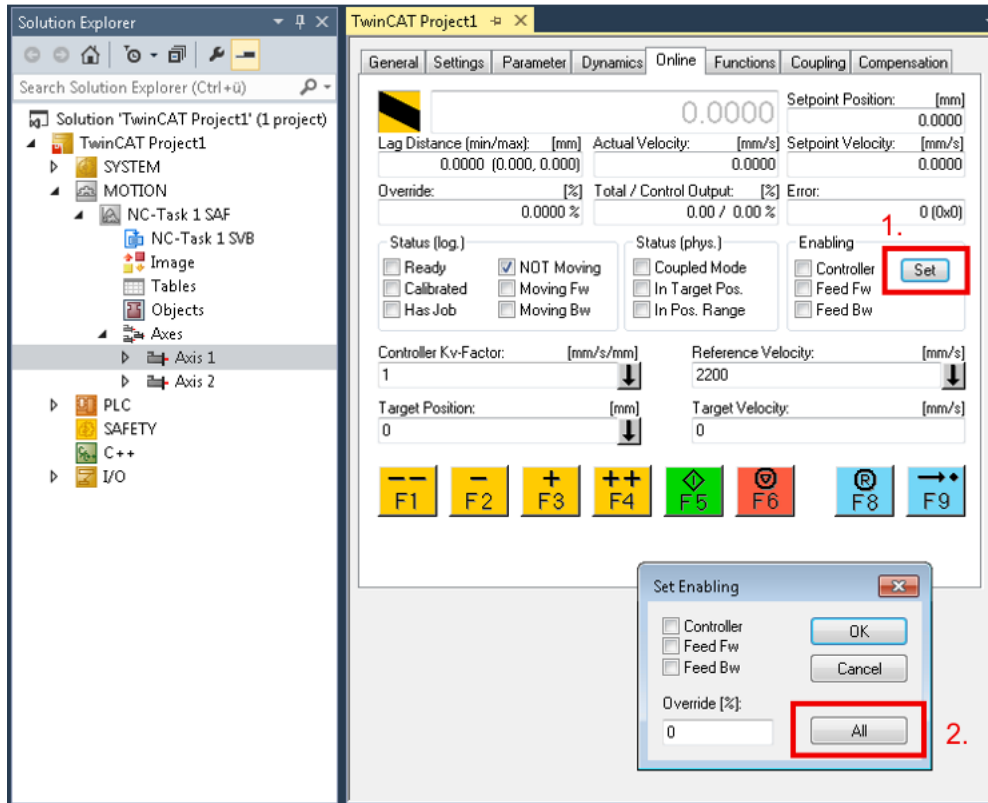
Fig. 20: Enabling an axis
