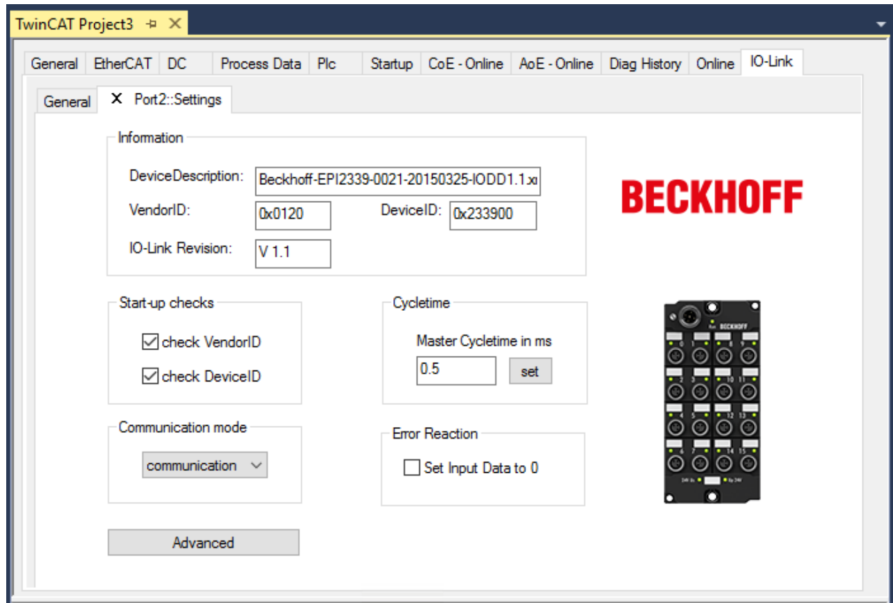
Abb. 19: Settings Device Port2
