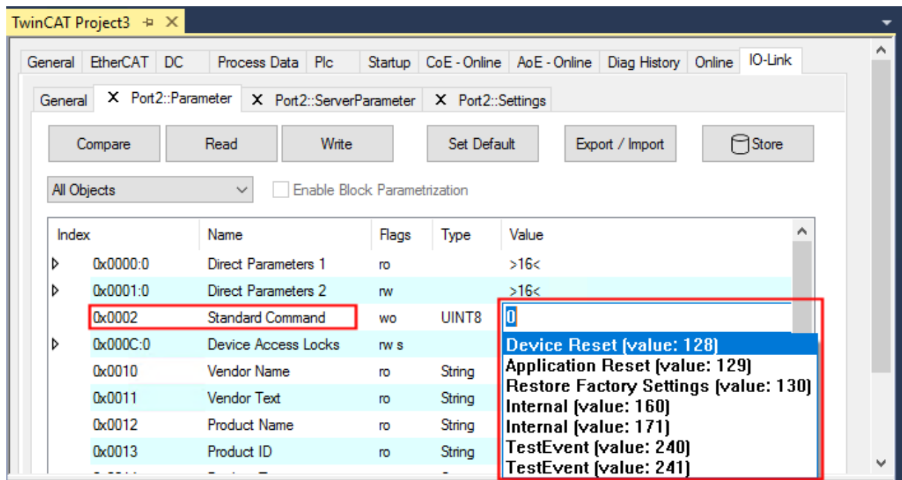
Abb. 36: IO-Link Device Parameter: "Standard Command"
