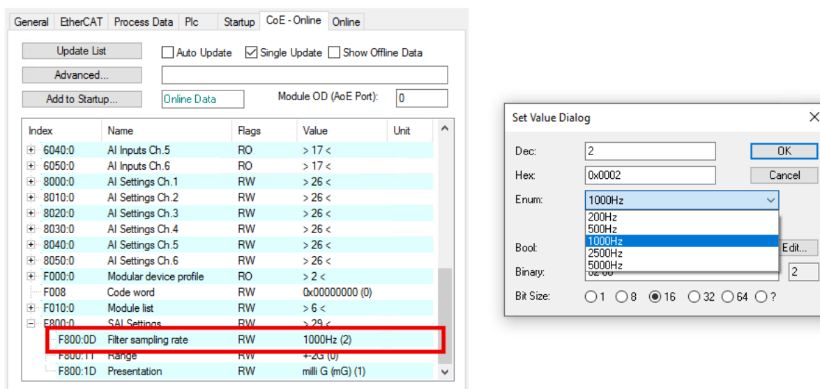
Fig. 6: Setting of the internal sampling rate (index 0xF800:0D)
