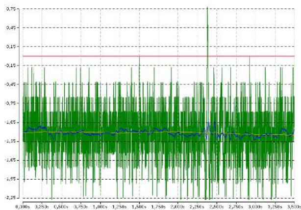
Fig. 8: Signal noise in detail
