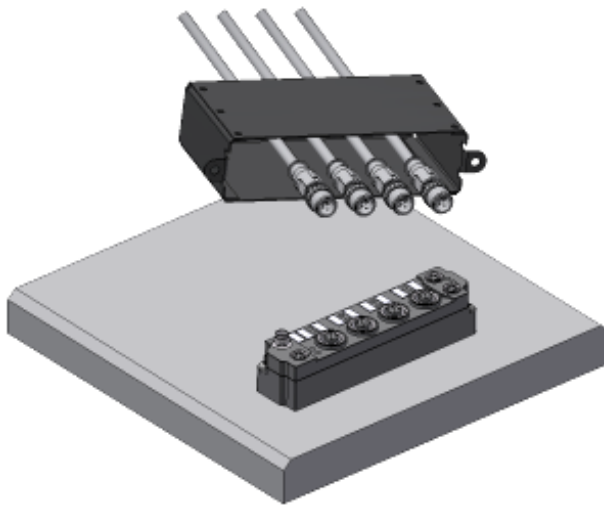
Fig. 12: BG2000-0000 - push the connecting cables through
