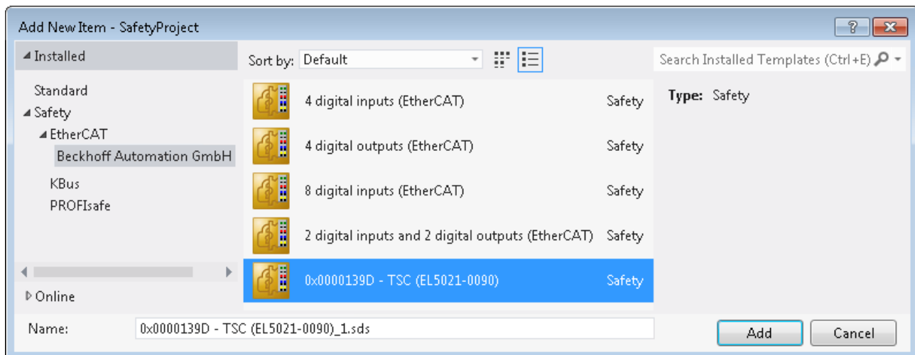
Fig. 20: Adding a TwinSAFE SC connection
