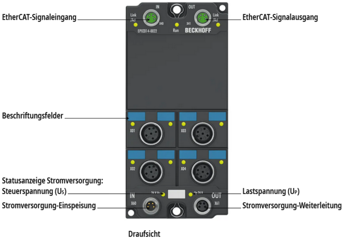
Abb. 2: EPX3314-0022 - EtherCAT Box, 4-Kanal-Analog-Eingang, Thermoelement, 16 Bit, M12, Ex i
