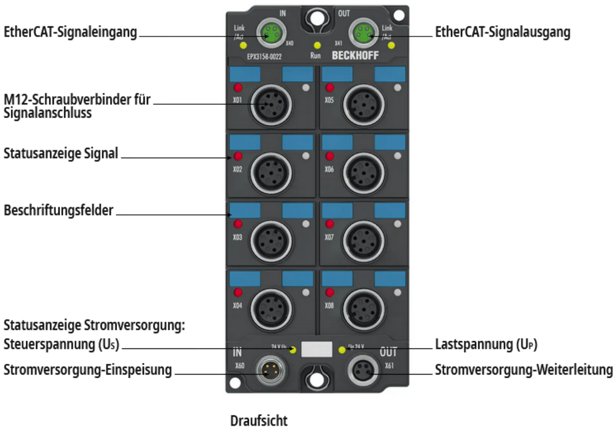
Abb. 2: EPX3158-0022 - Achtekanalige, analoge EtherCAT Box, 4...20 mA, single-ended, 16 Bit, Ex i
