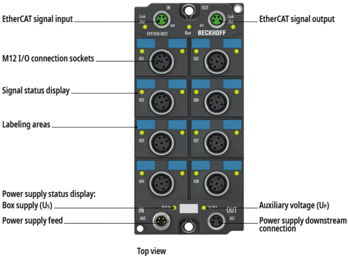
Fig. 2: EPX1058-0022 - 8-channel digital EtherCAT Box for NAMUR sensors, Ex i
