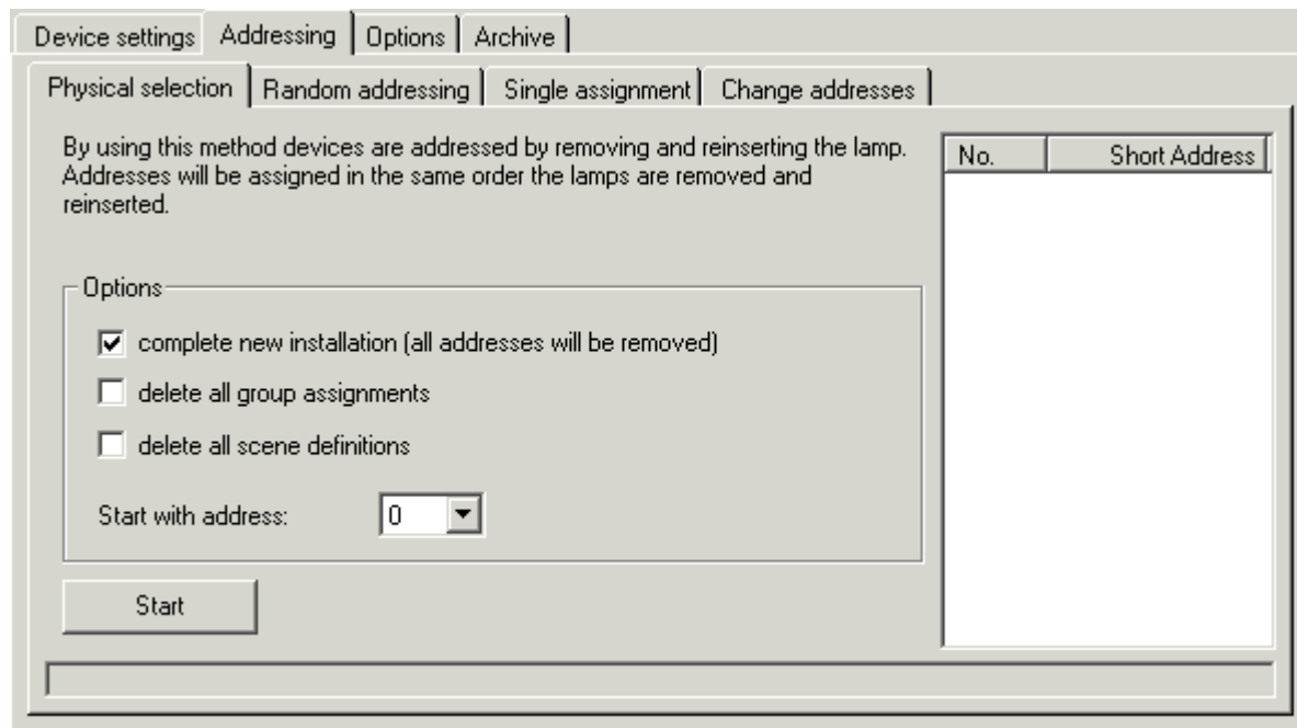
Fig. 24: KS2000 - addressing of the DALI device - physical selection
