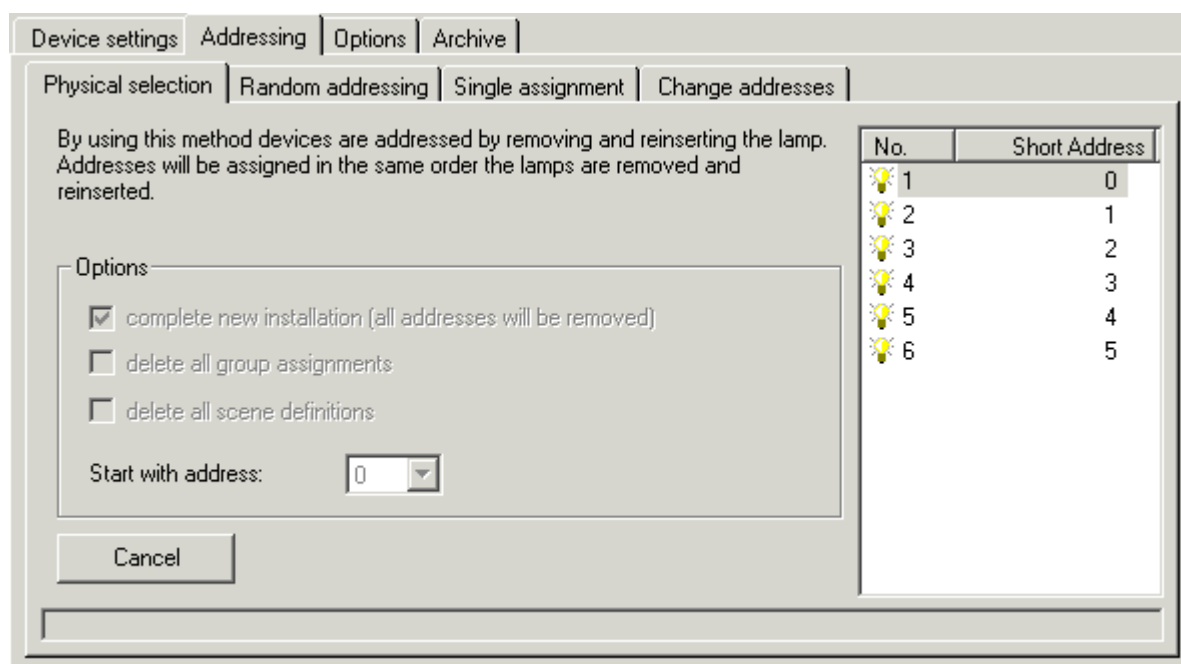
Fig. 25: KS2000 - addressing of the DALI device - displaying the physical addressing
