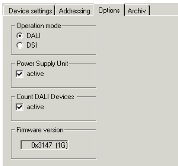
Fig. 30: KS2000 - Options for the KL6811
