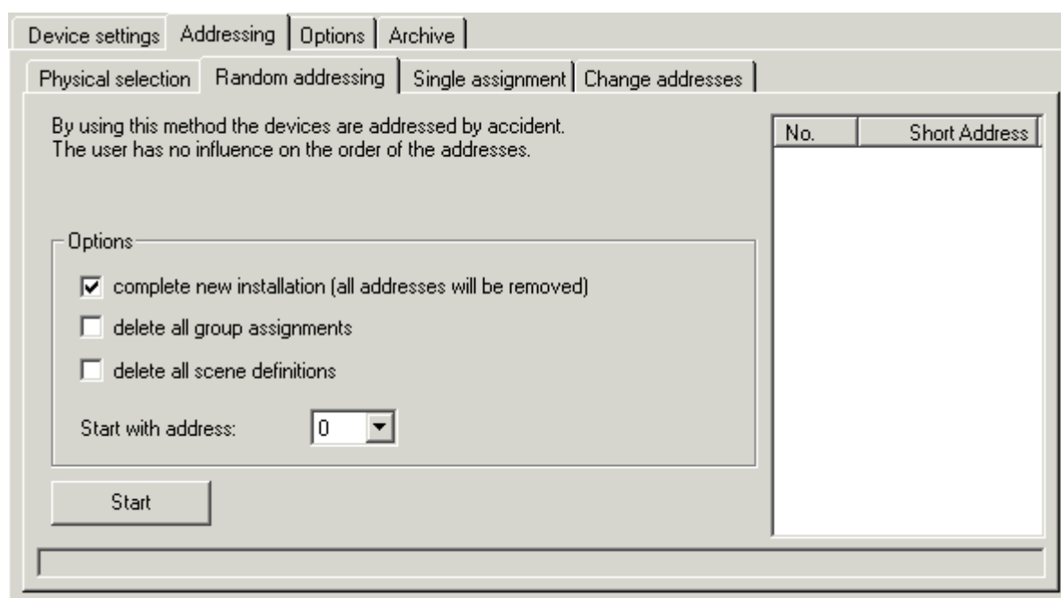
Fig. 26: KS2000 - addressing of the DALI device - random addressing
