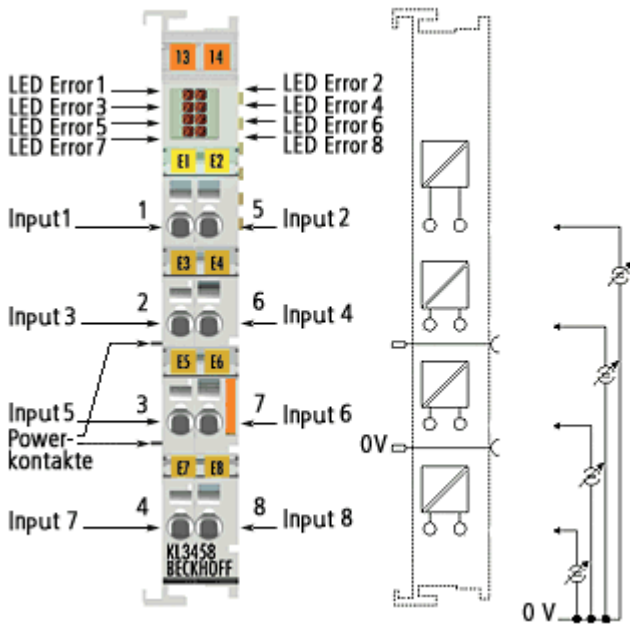
Abb. 7: KL3458
