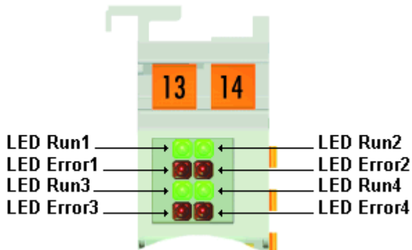
Abb. 5: KL3444, KL3454 - Diagnose-LEDs
