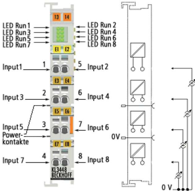
Abb. 6: KL3448
