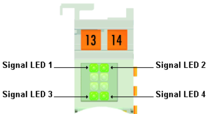
Abb. 3: LEDs
