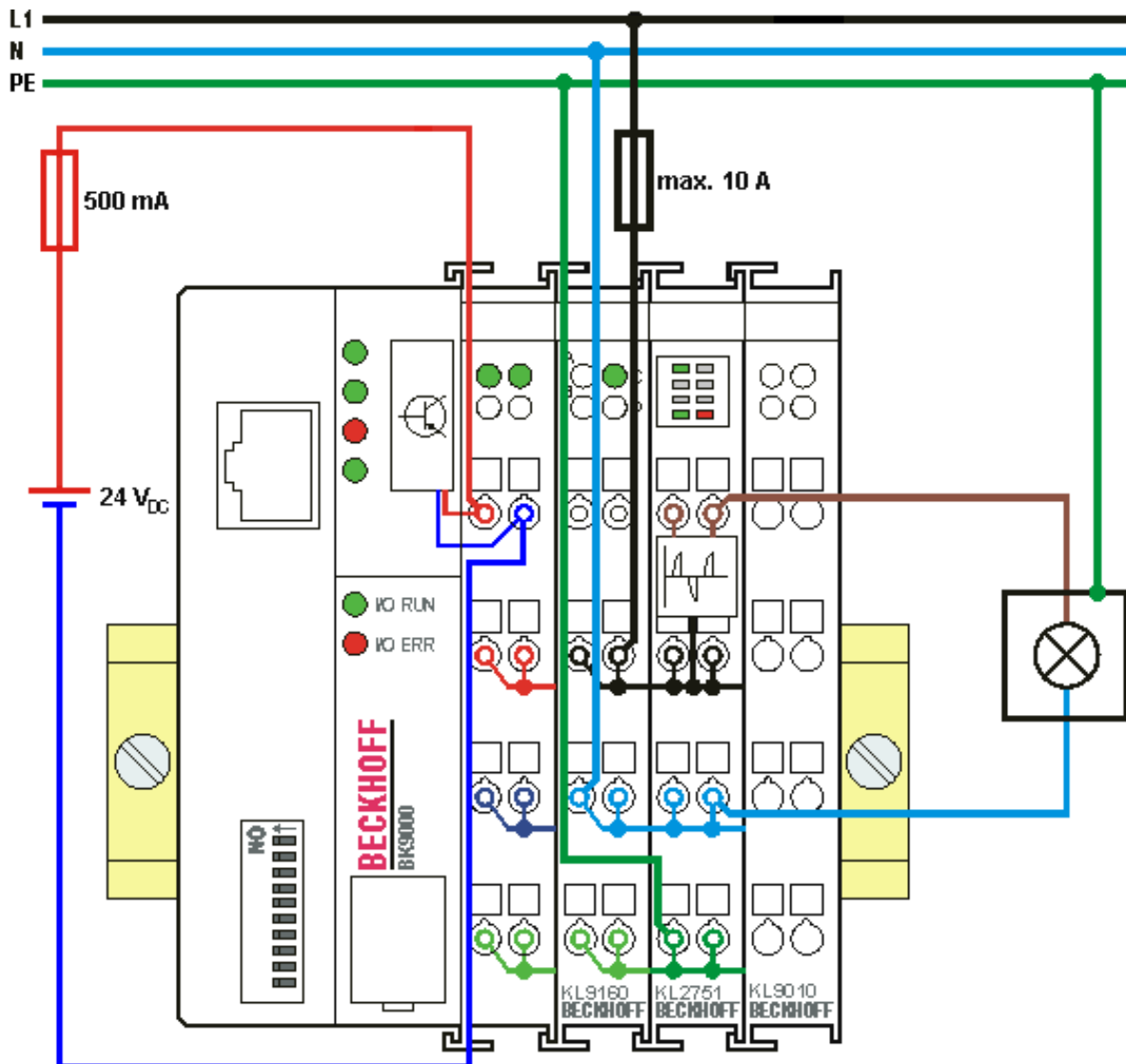
Fig. 16: KL2751 - Application example
