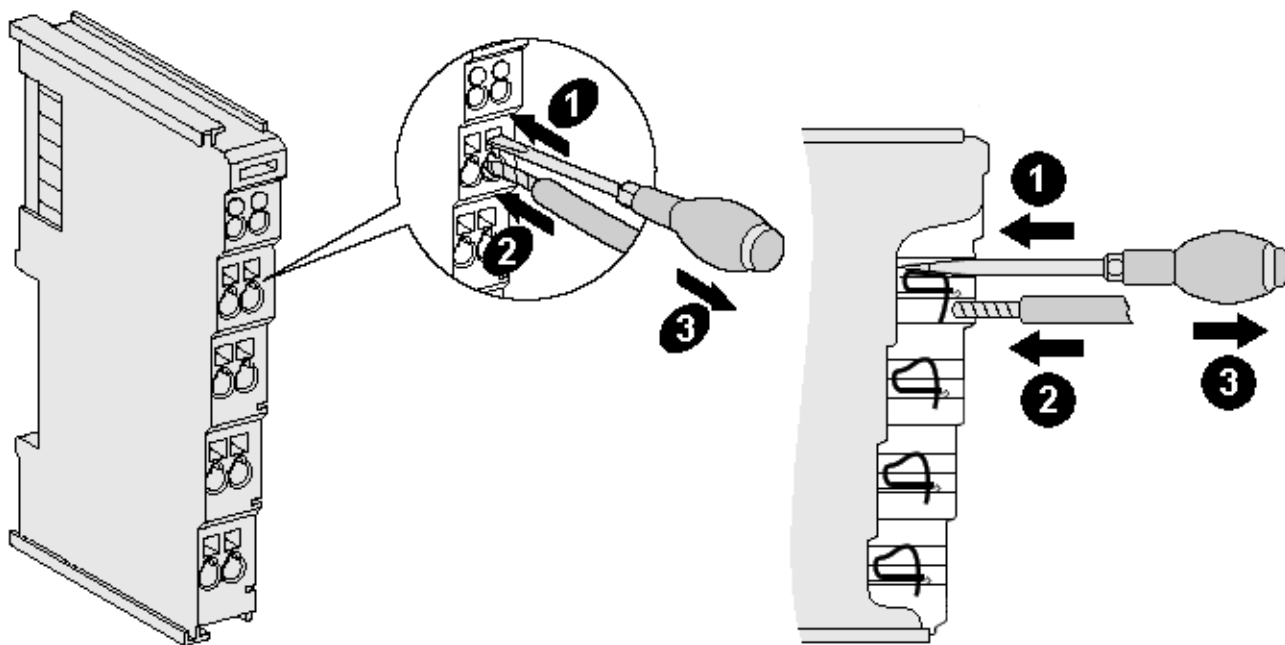
Fig. 14: Connecting a cable on a terminal point
