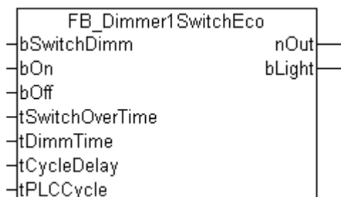
Fig. 28: FB_Dimmer1SwitchEco
