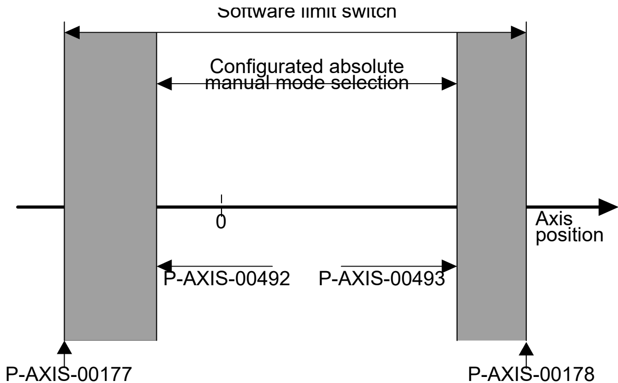
Fig. 38: Absolute motion limits in manual mode
