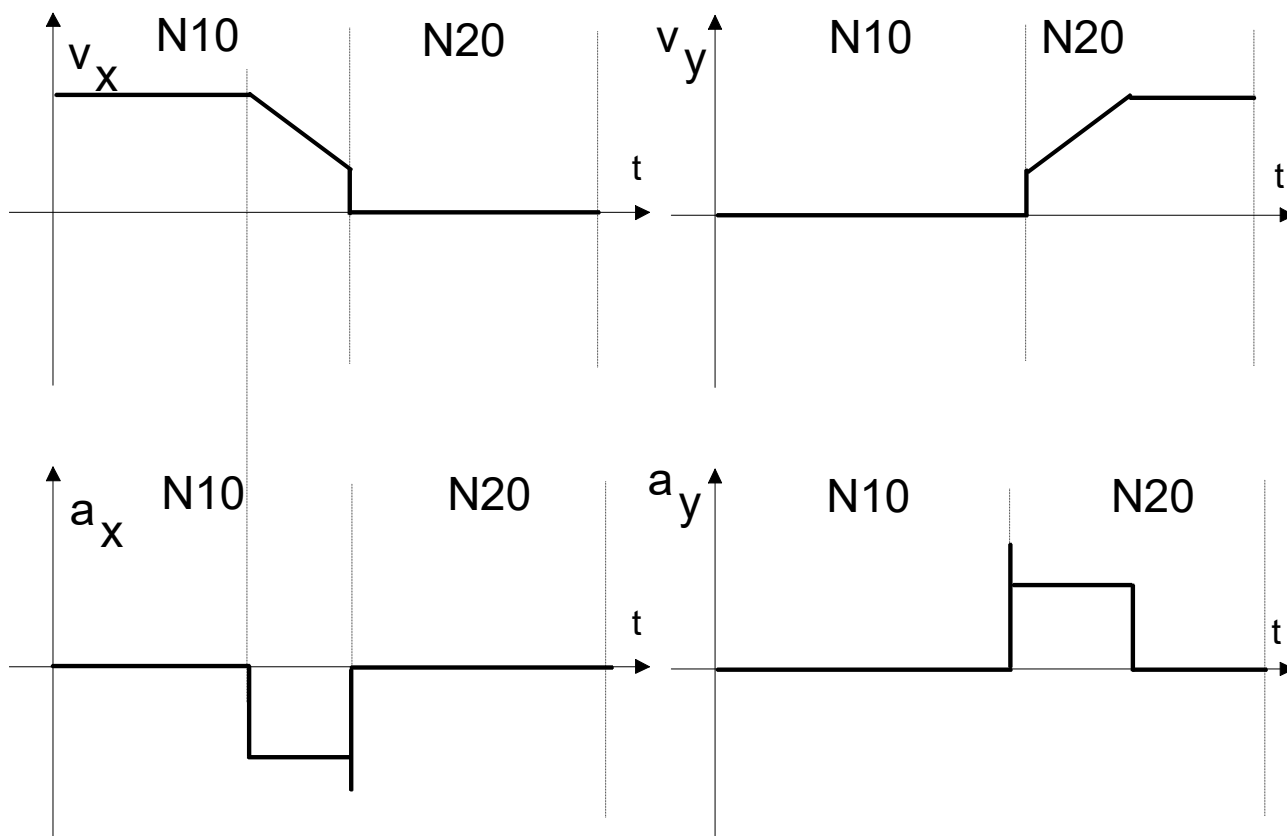
Fig. 21: Acceleration at linear-linear block transition
