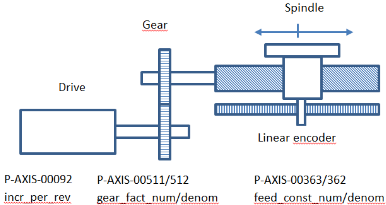
Fig. 55: Position scaling with linear encoder
