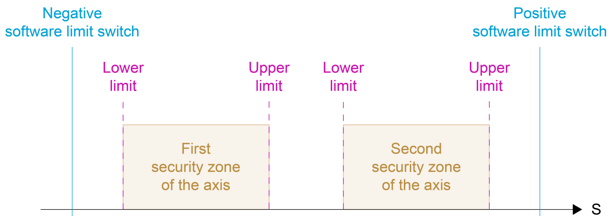
Fig. 9: Representation of 2 security zones and limits of an axis
