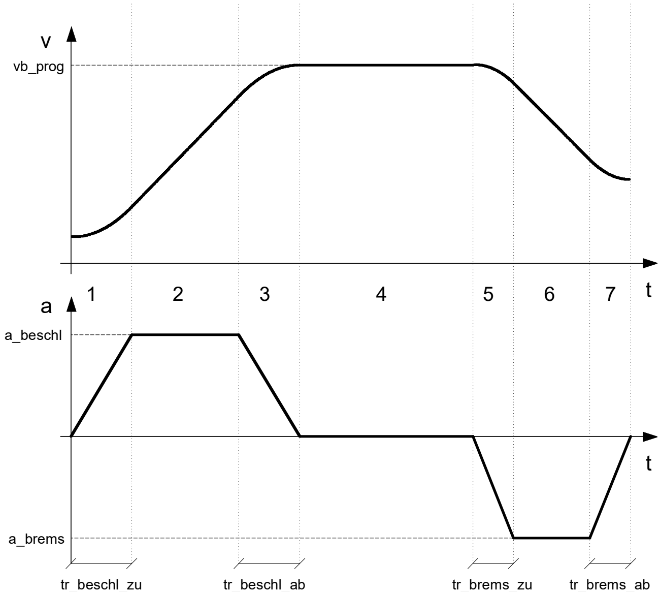
Fig. 18: Non-linear velocity profile
