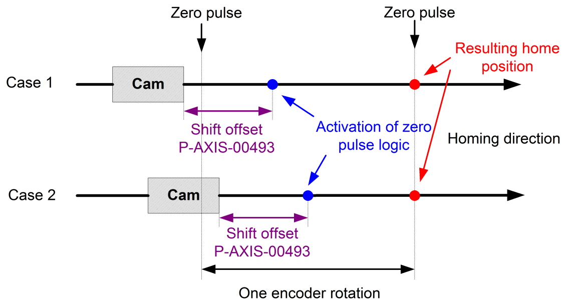
Fig. 5: Reliable detection of identical zero impulse positions
