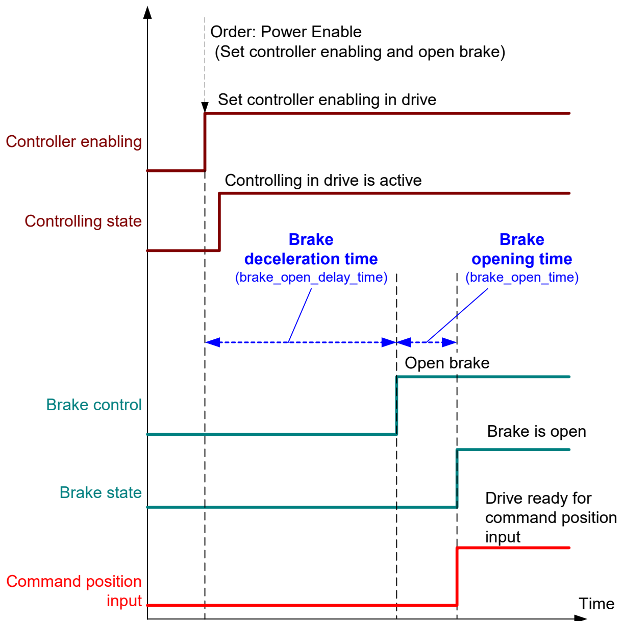
Fig. 36: Timing opening the brake
