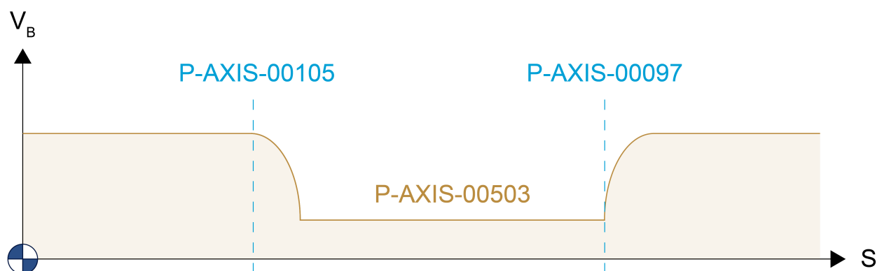
Fig. 11: Parameters of permissible axis velocities inside the second security zone
