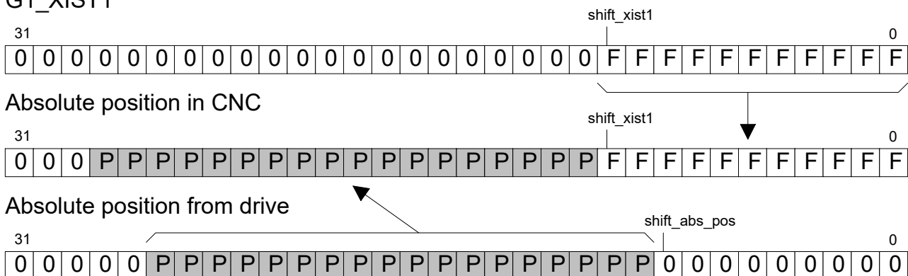
Fig. 35: Calculation mode for encoder actual position for additive encoder
