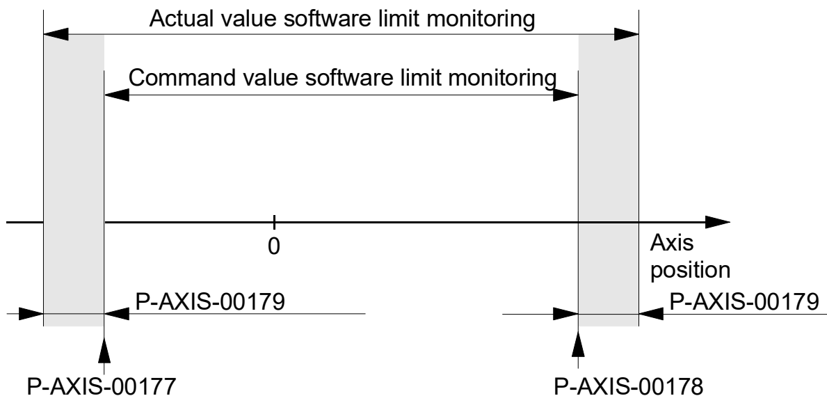
Fig. 6: Monitoring of command and actual values for software limit switch.
