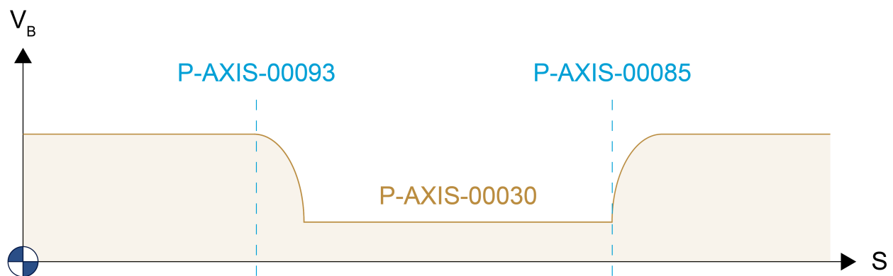
Fig. 10: Parameters of permissible axis velocities inside the security zone 1
