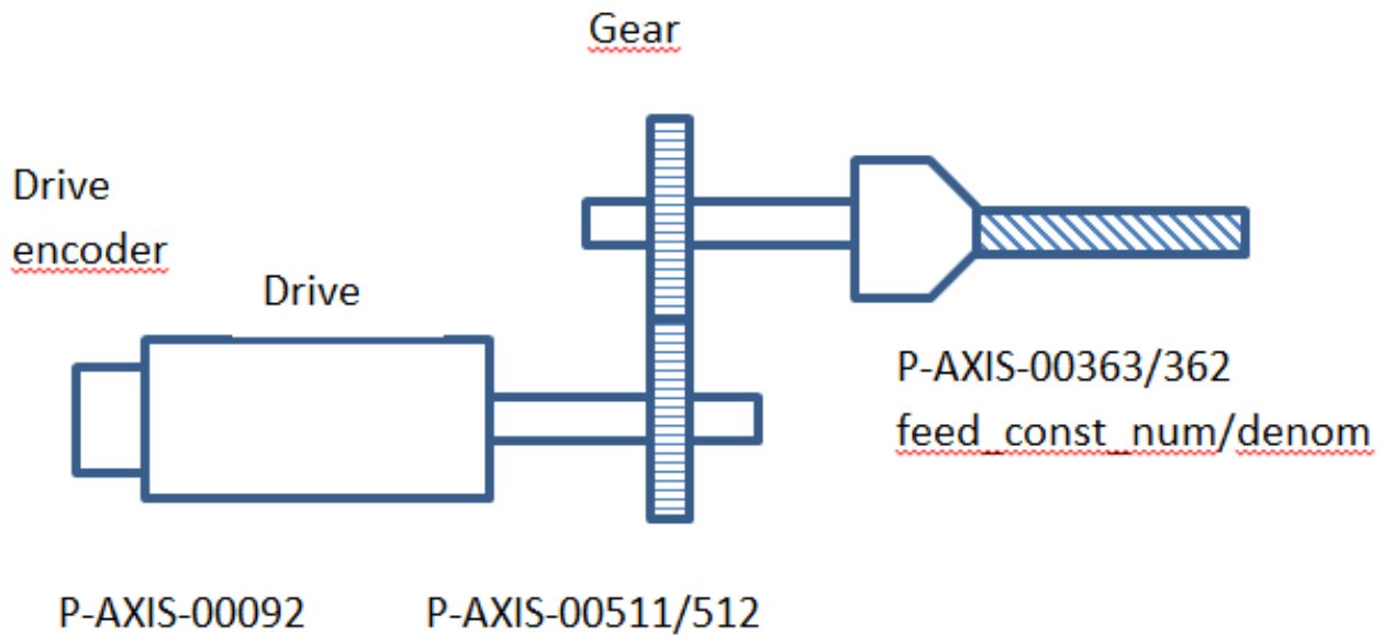
Fig. 56: Position scaling with fitted encoder
