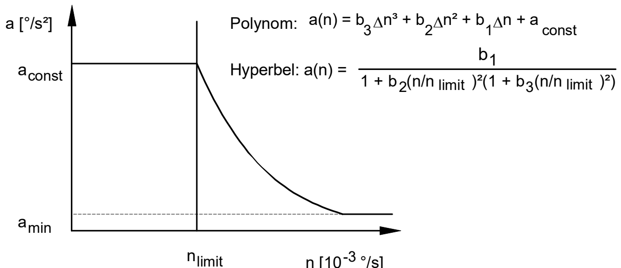
Fig. 25: Characteristic a(n) in polynomial or hyperbolic form
