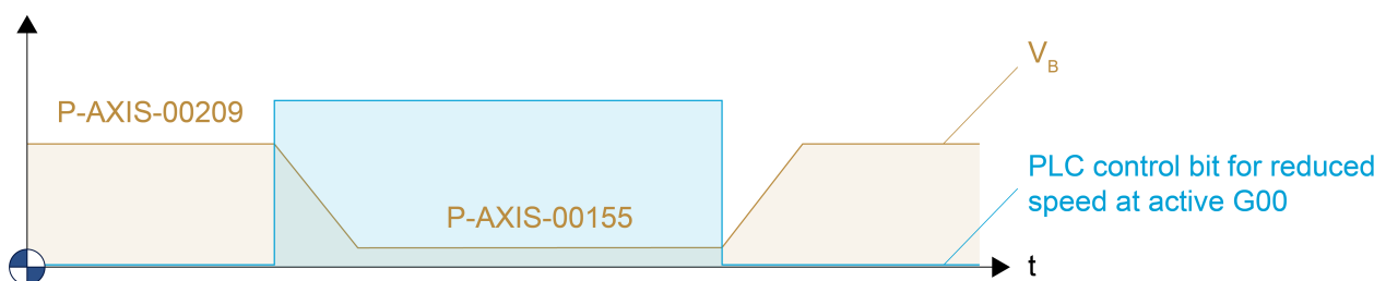
Fig. 8: Reduced maximum speed with active G00
