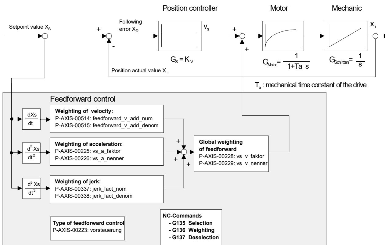
Fig. 31: Block diagram of feedforward control
