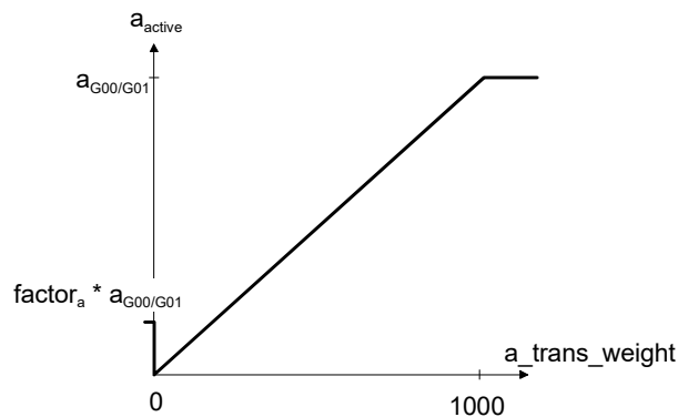
Fig. 22: Factor range for acceleration weighting at block transition
