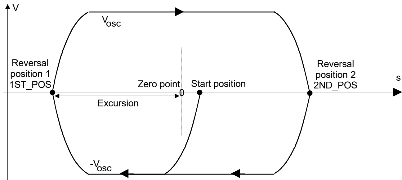
Fig. 16: Positioning procedure with pendulum movement
