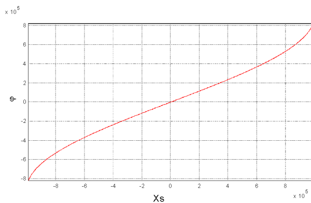
Fig. 44: Graphic diagram of the eccenter function
