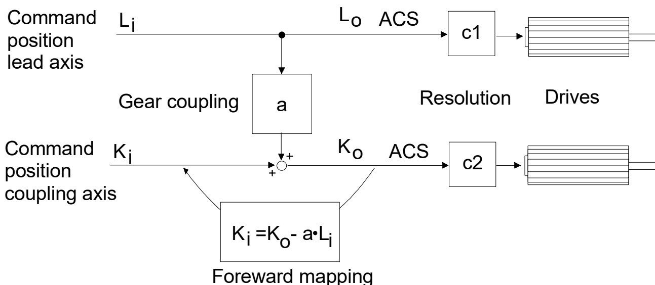
Fig. 13: Principle of electronic gear coupling
