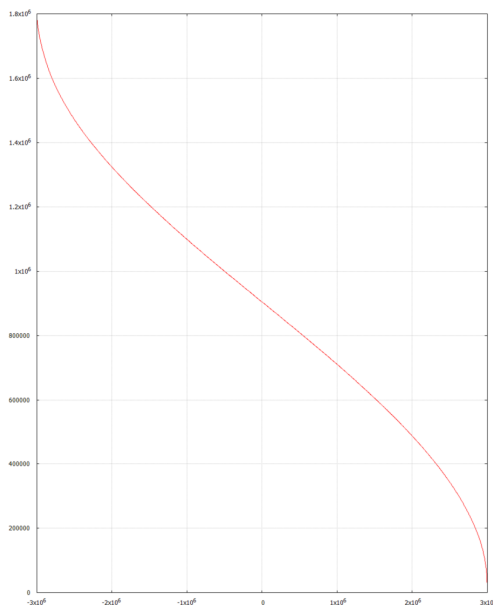
Fig. 52: Transfer function of the symmetrical slider crank
