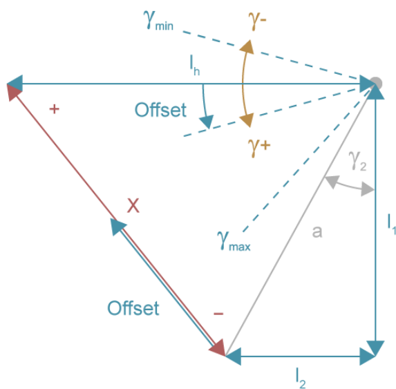
Fig. 48: Angular kinematic
