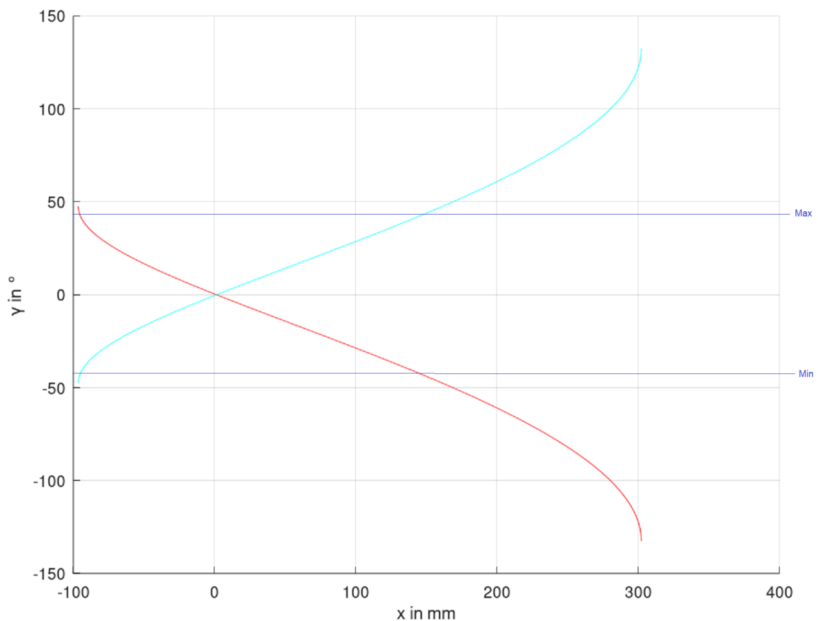
Fig. 50: Transfer function with and without angle inversion
