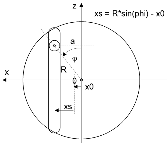
Fig. 43: Kinematic diagram of the eccenter function
