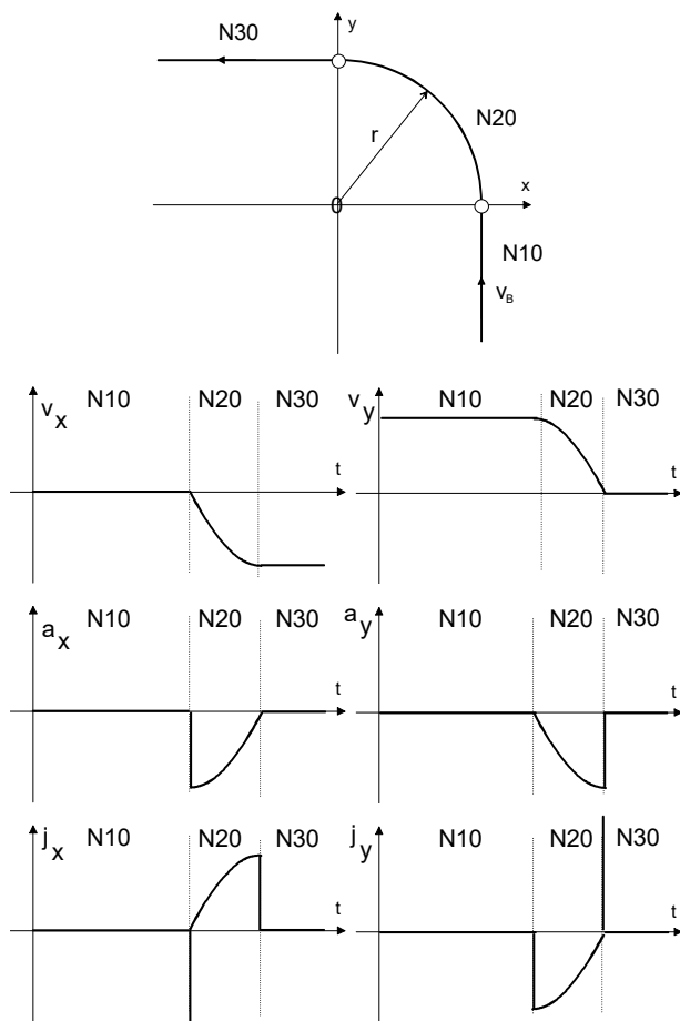
Fig. 23: Acceleration and jerk at linear-circular block transition
