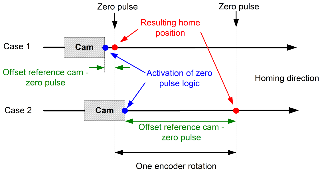
Fig. 4: Detection of different zero impulse positions possible
