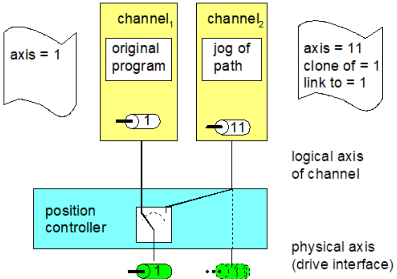
Fig. 1: Configuration of physical and logical axes
