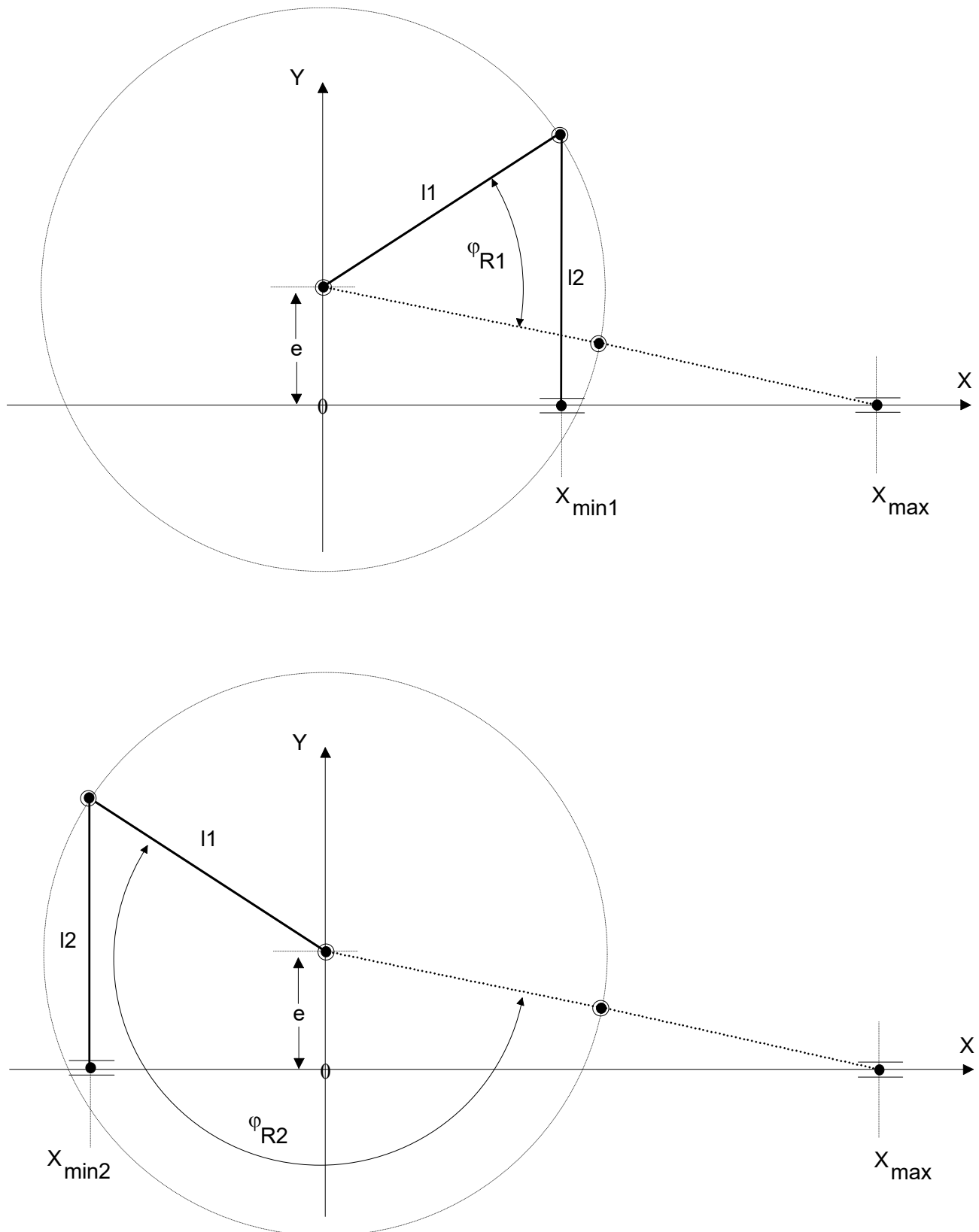
Fig. 42: Extreme positions of slider crank with eccentricity
