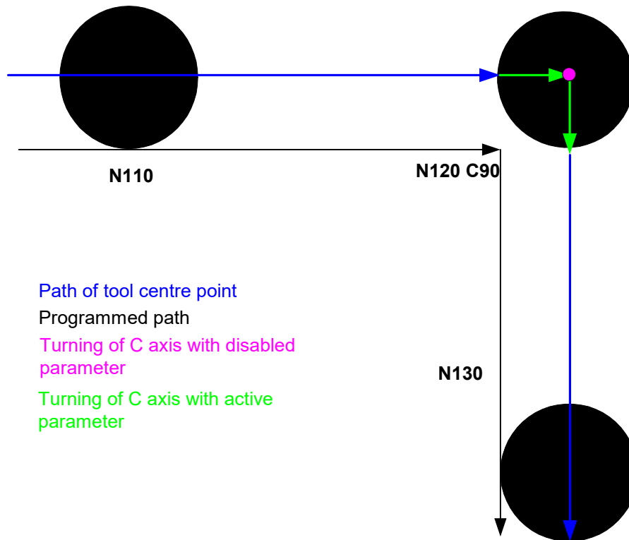
Fig. 15: Principle motion sequence of a C axis with G25
