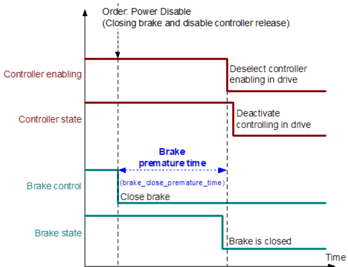
Fig. 37: Timing when closing the brake
