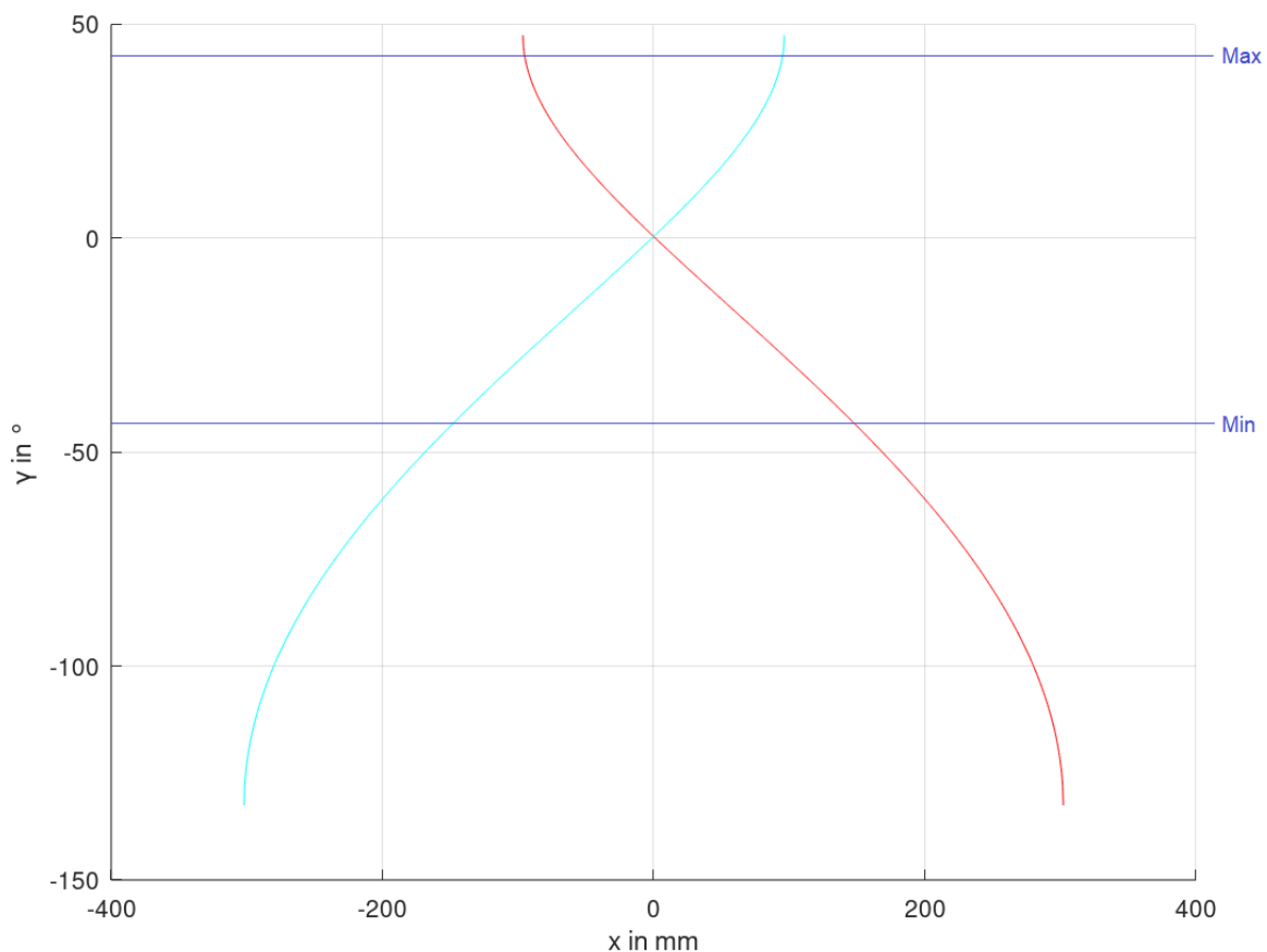
Fig. 51: Transfer function with and without linear position inversion
