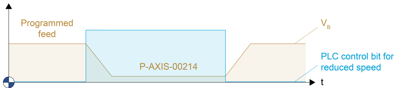
Fig. 7: Reduced maximum speed with active G01
