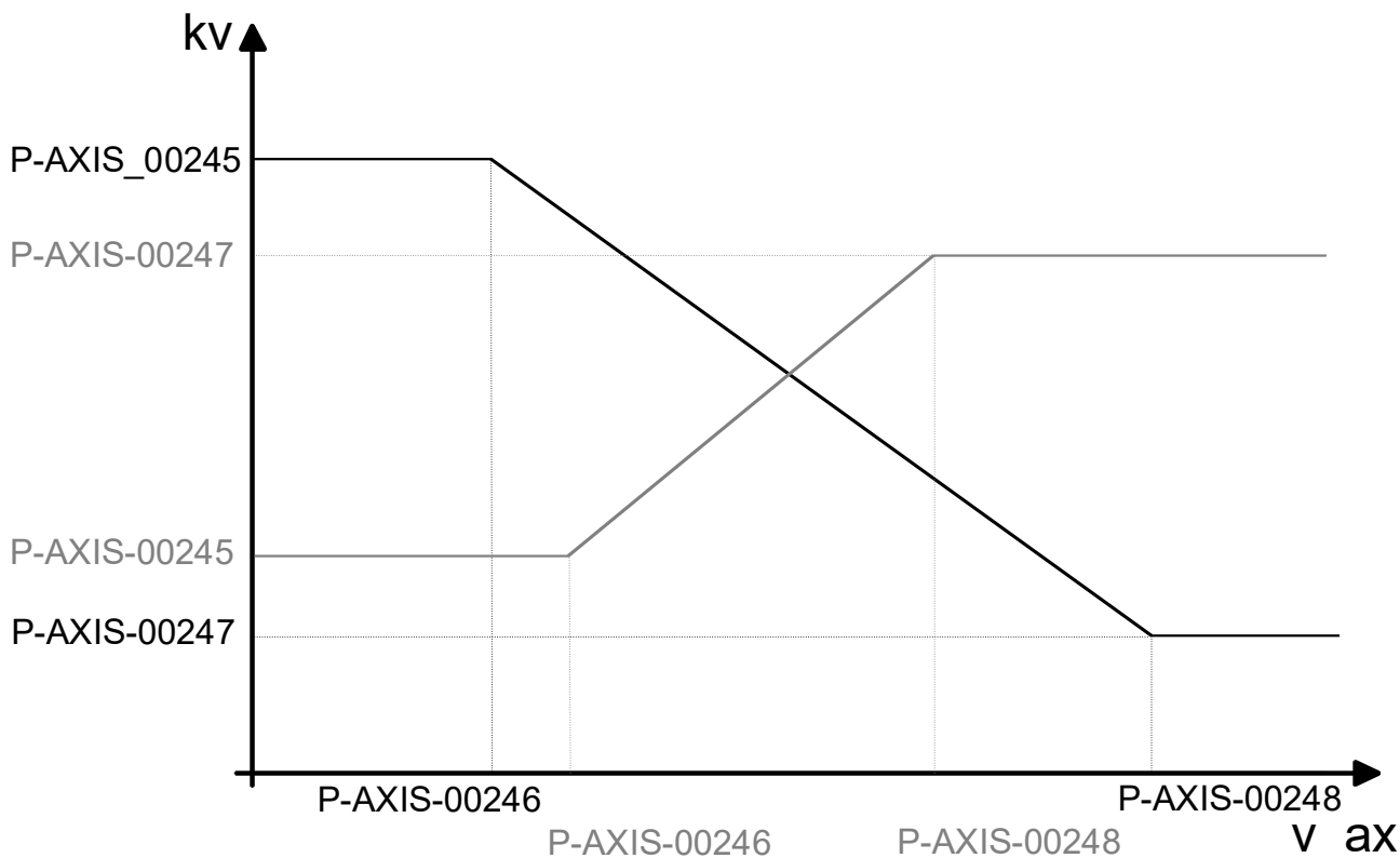
Fig. 29: Parameters of dynamic kv adjustment
