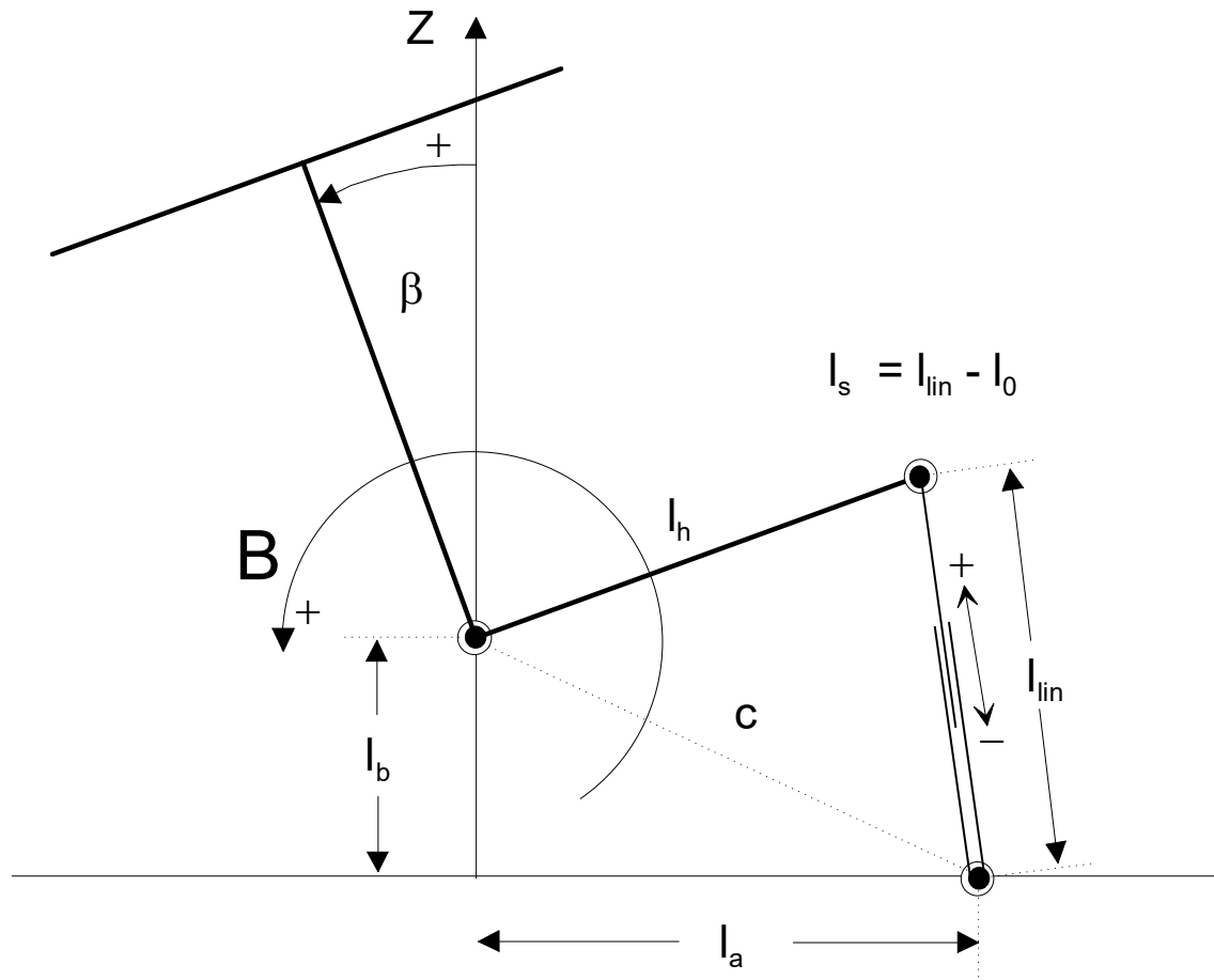
Fig. 45: Kinematic structure of crank and linkage
