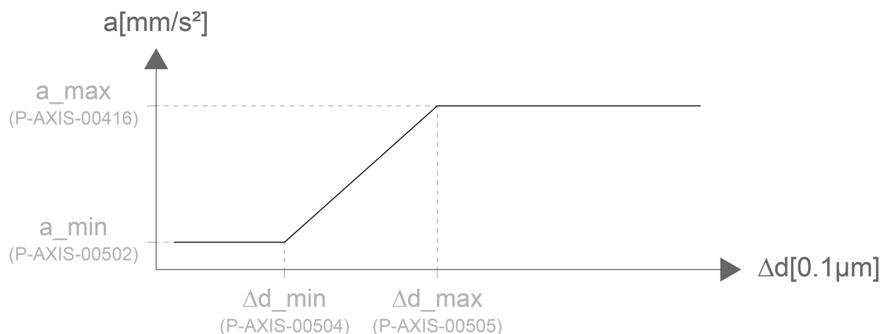
Fig. 30: Parameters for acceleration and distance error
