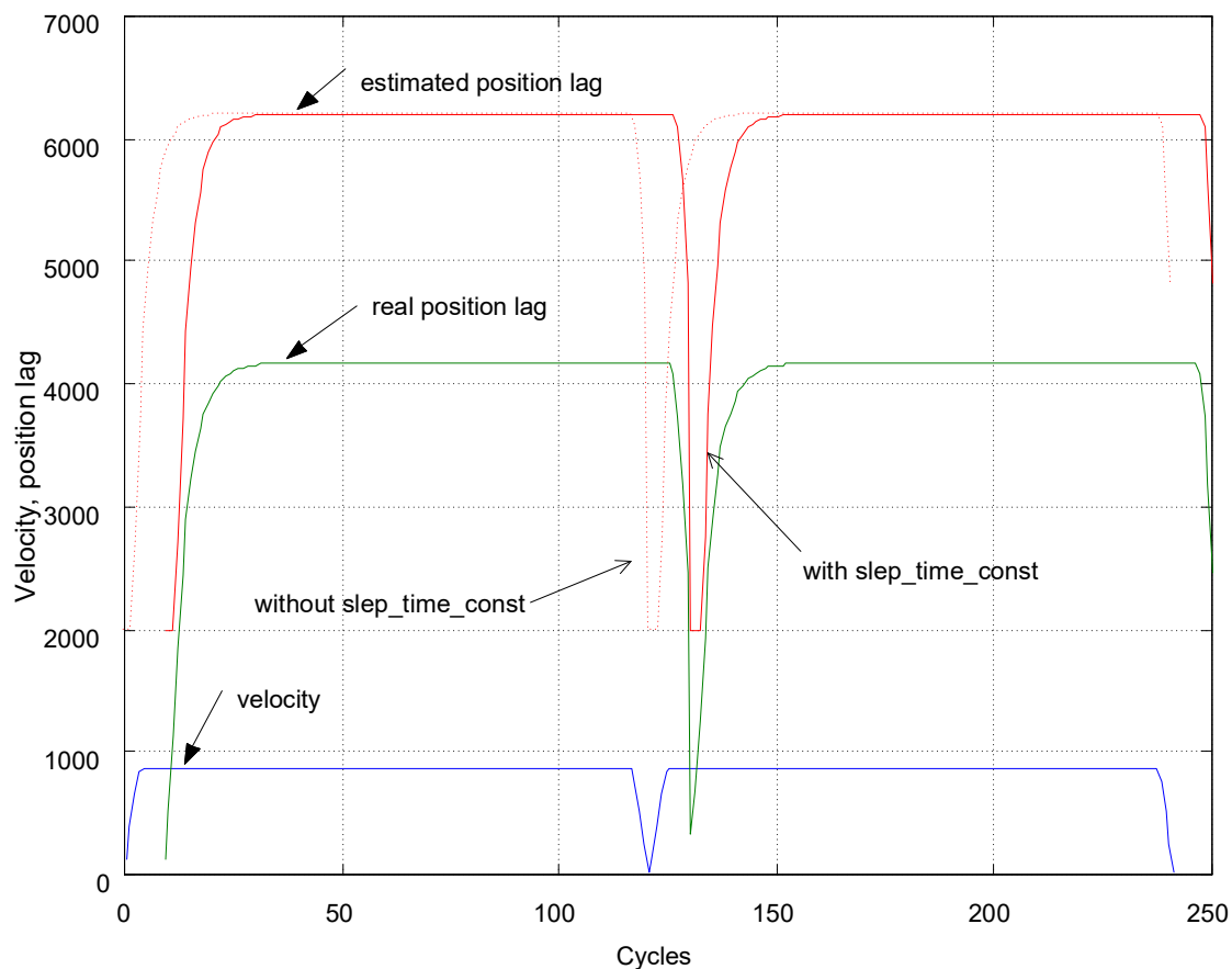
Fig. 28: Time constant to shift monitoring curve
