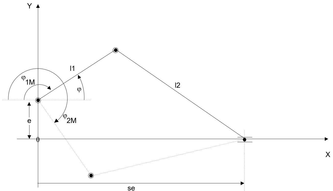
Fig. 40: Kinematic structure of slider crank
