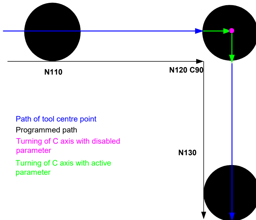
Fig. 14: Principle motion sequence of a C axis with G26
