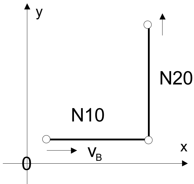
Fig. 20: Acceleration by block transitions N10 to N20 due to a direction change
