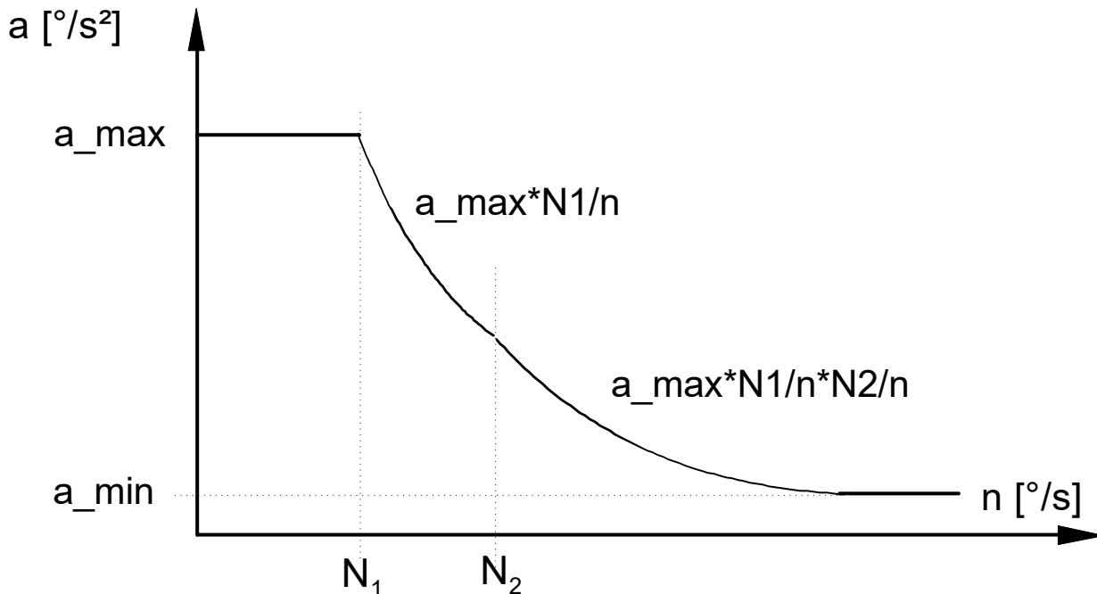
Fig. 26: Characteristic curve for asynchronous drives
