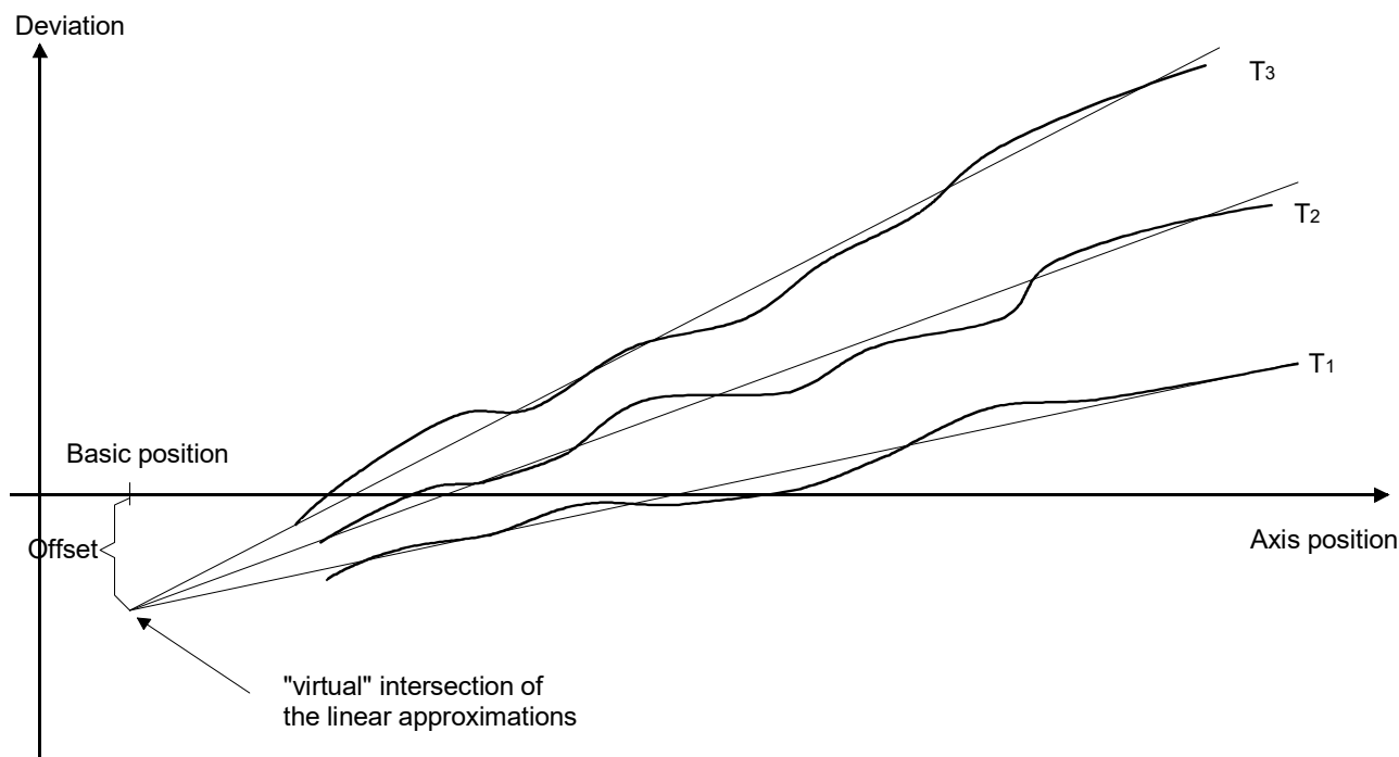
Fig. 27: Reference measurement at different temperatures
