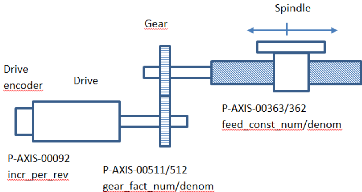
Fig. 54: Position scaling with rotary encoder
