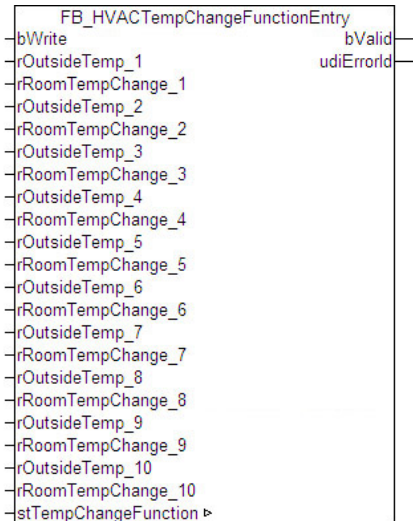
Abb. 19: FB_HVACTempChangeFunctionEntry
