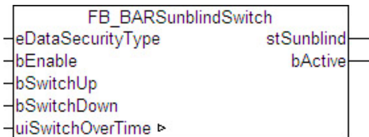
Abb. 9: FB_BARSunblindSwitch
