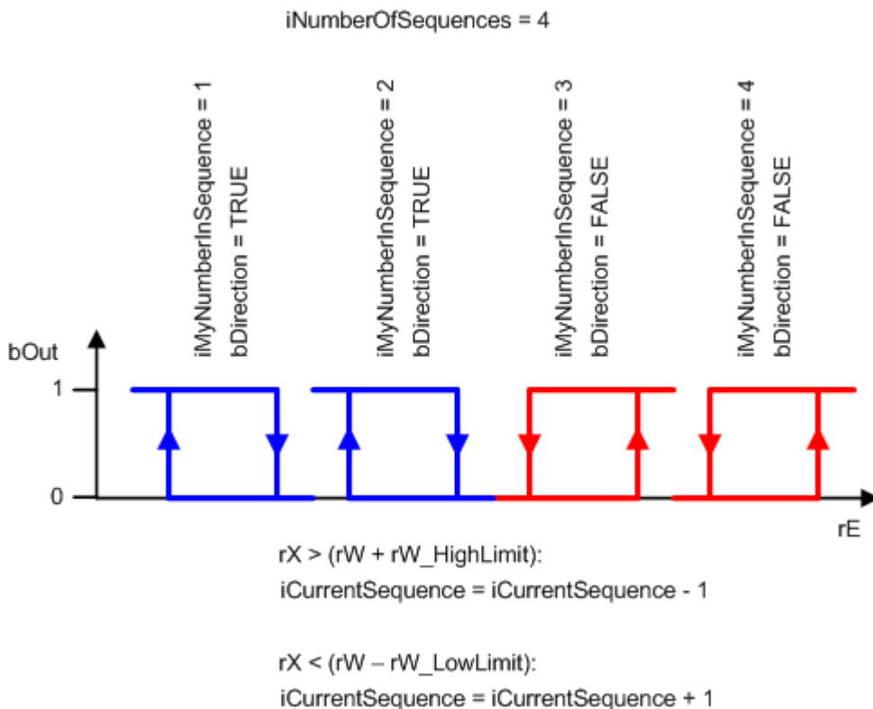
Abb. 16: FB_HVAC2PointCtrlSequence_1
