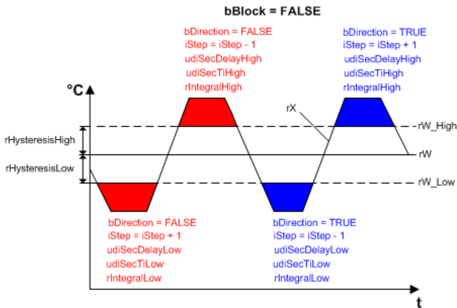
Abb. 13: FB_HVACI_CtrlStepParameter
