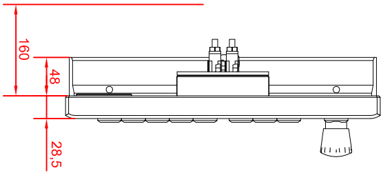
left view
