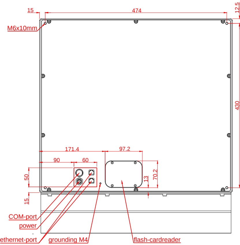
rear view
