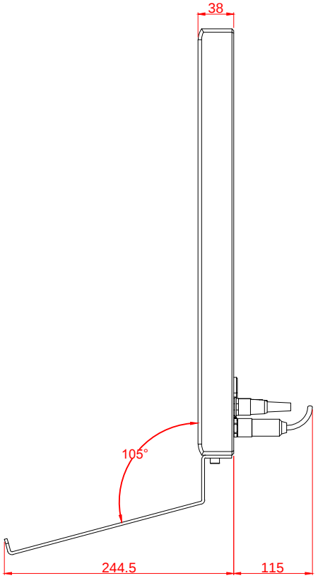
left view
